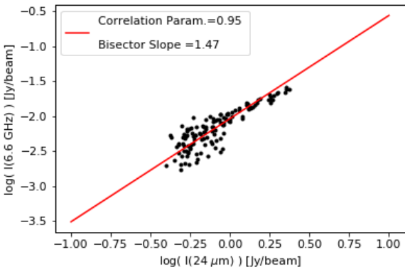
Fig. 25. Upper panel: 24 \mu\text{m} –radio correlation for pixels within the 10 kpc star forming ring. The log-log slope for the ring is 0.73 \pm 0.01 . Lower panel: same correlation as in the top panel but for pixels within the central region. The log-log slope for the central region is 1.47 \pm 0.04 . Only pixels above 3\sigma have been used.
