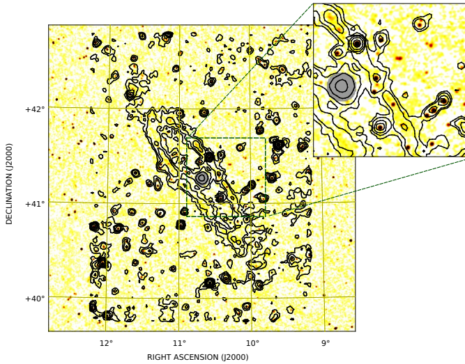
Fig. 2. NVSS image at 1.4 GHz with the SRT contours at 6.6 GHz. Levels start at 2 \text{ mJy beam}^{-1} and increase by a factor of two. The inset shows a detail of the M31 ring. The extended emission of the central region (grey area) has been excluded from the point-source search.
