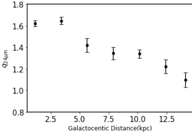
Fig. 30. q_{24\mu\text{m}} parameter vs. galactocentric distance.
