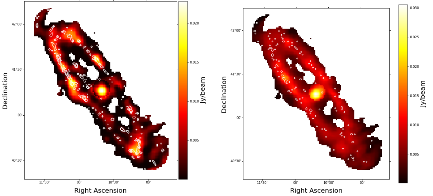
Fig. 18. Left panel: thermal (free-free) emission map at 6.6 GHz with HII contours. Contour levels indicate 2, 3, 6, 9, and 12 HII regions inside the C-band pixel. Right panel: same as left panel, but for the synchrotron component (nonthermal) with SNR contours. Contour levels show 1, 2, and 3 SNRs inside the C-band pixel. The resolution of both thermal and nonthermal maps is 5'.
