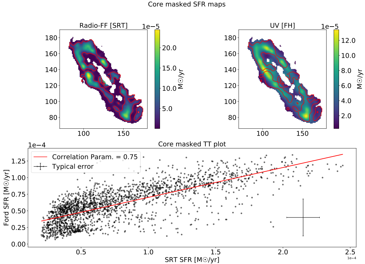
Fig. 22. T-T plot between the radio-free-free SFR map and the F13 map with the central area masked. The red contours on the top two maps highlight the regions with S/N > 3 in our SFR map ( top-left panel ), and therefore the pixels that have been considered in this analysis. The plot shows a good correlation between the two maps in the ring region with a correlation parameter of r_{\text{ring}} = 0.75 .
