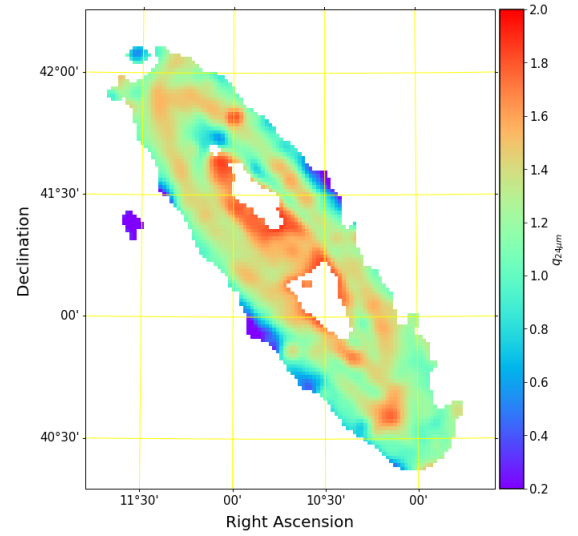
Fig. 29. Logarithmic IR–radio ratio map obtained with EFF20 and Spitzer 24 \mu\text{m} maps, both convolved to 3' .
