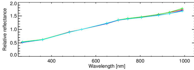
(c) Spectrophotometric plots for the selected features of obs. ID 1
