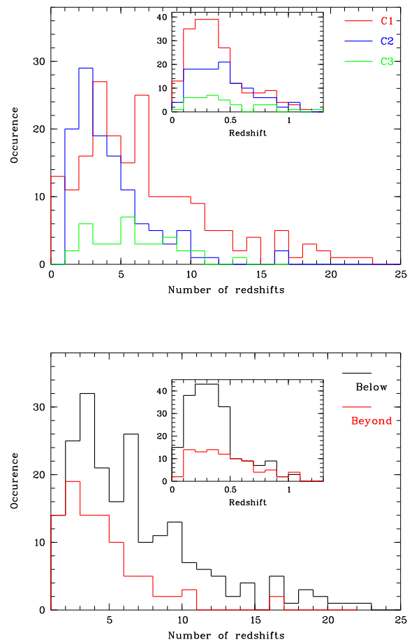
Fig. 6. Distribution of the number of spectroscopic redshifts inside clusters with a redshift estimate. The insets show the redshift histograms of these samples. Top panel: C1 (red histograms), C2 (blue histograms), and C3 (green histograms) clusters. Bottom panel: clusters with also a flux estimate fainter (black histograms) and brighter (red histograms) than the reference flux completeness limit of 1.3 \times 10^{-14} \text{ erg s}^{-1} \text{ cm}^{-2} .
