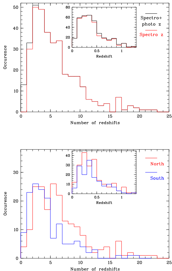
Fig. 5. Distribution of the number of spectroscopic redshifts inside clusters with a redshift measurement. The insets show the redshift histograms of these samples. Top panel: Spectroscopic + photometric redshift sample (black histograms), and spectroscopic redshift sample (red histograms) clusters. Bottom panel: XXL-N (red histograms) and XXL-S (blue histograms) clusters. Photometric redshifts are used in replacement of spectroscopic redshifts in these two histograms when spectroscopic redshifts are not available.
