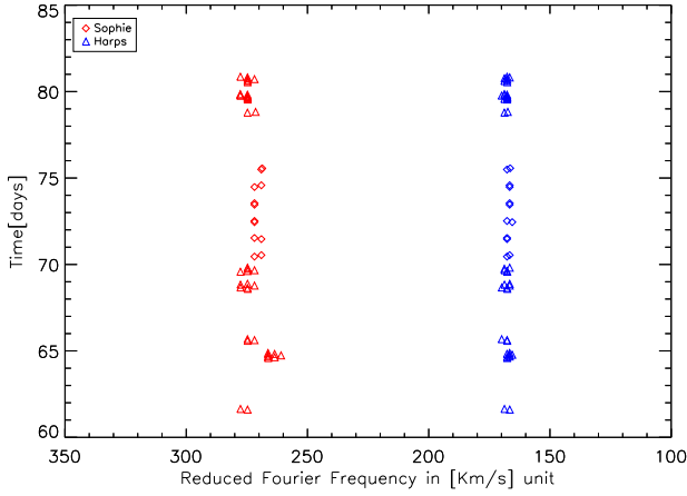
Fig. 10. Position of the first (red) and second (blue) minima of He I \lambda 4471 Fourier-transform profiles of HARPS and SOPHIE spectra.
