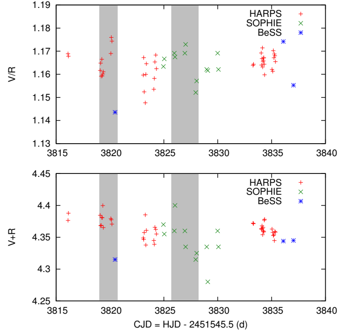
Fig. 5. Violet over red ( V/R ) emission ratio (top panel) and sum of the V and R emission (bottom panel) measured in the emission peaks of the H\alpha line observed with HARPS, SOPHIE, and additional spectra from the BeSS database. The hashed regions indicate the occurrence of minor outbursts.
