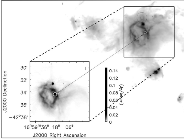
Figure 5. Composite picture of the field centred on [DBS2003] 176. The sub-panel on the bottom-left corner shows the SCORPIO map, while the background is the FIR map from Herschel (PACS, 70 \mu m). The arrow indicates the position of the compact component SCORPIO1_300. The dotted circle in the background FIR map highlights the position of the bubble S16 (see text). In the online version a colour figure is available where the background panel is an RGB false colour image obtained from the composition of the mid-IR/FIR maps from Spitzer (IRAC, 8 \mu m, green) and Herschel (PACS, 70 \mu m, red) with the SCORPIO map (blue).
