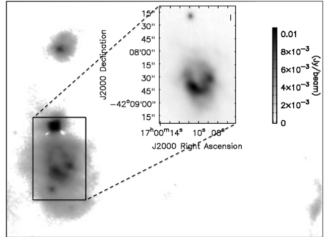
Figure 6. Composite picture of the field around IRAS 16566-4204. The sub-panel on the top-right corner shows the SCORPIO map, while the background is the FIR map from Herschel (PACS, 70 \mu m). In the field two radio sources are visible. The point-like source is associated with SCORPIO1_600, while the more extended source is associated with SCORPIO1_592a and SCORPIO1_592b. A colour figure is available in the online version of the paper. The colour code of the online figure is described in the caption of Fig. 5.
