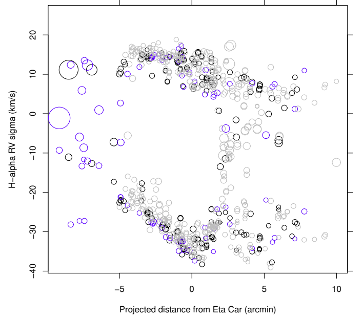
Fig. 33. Same as Fig. 32, except that circle size is proportional to line width \sigma .
