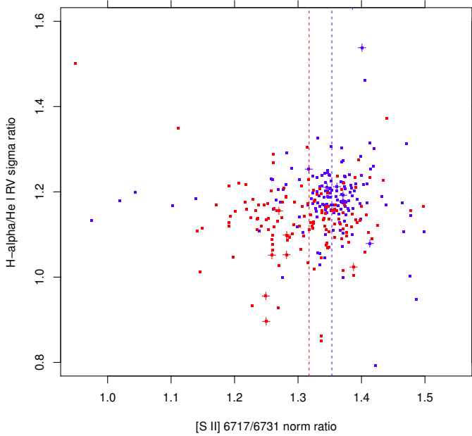
Fig. 15. Gaussian width ratio between Hα and He I (proxy for temperature) vs. normalization ratio between [S II] 6717/6731 Å (proxy for density). Temperature increases upwards, while density increases towards the left. Symbols are as in Fig. 7. The red (blue) vertical dashed line indicates the median [S II] 6717/6731 Å ratio for the receding (approaching) components. On average, the receding component has higher density and lower temperature than the approaching component.
