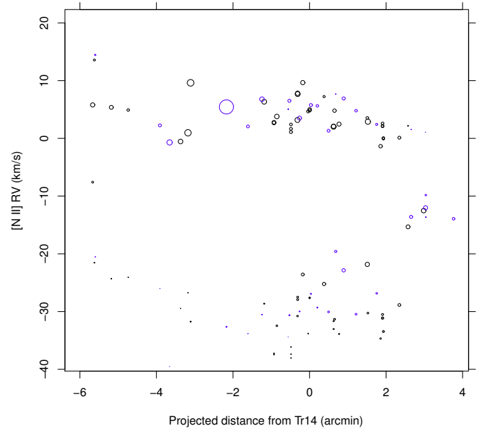
Fig. 31. Same as Fig. 29, but using the [N II] 6584 Å line.
