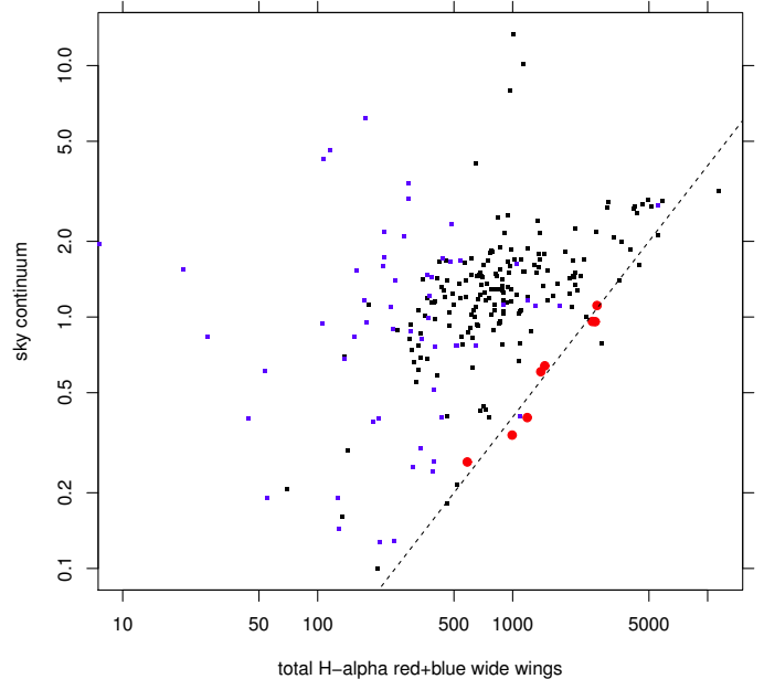
Fig. 19. Sky continuum vs. total intensity in the wide H\alpha wings. Small dots refer to pure-sky fibers from setups HR15N (black) and HR14A (blue), while big red dots are the downscaled continuum and wide wings of \eta Car. The dashed line is a constant factor of 4 \times 10^{-4} .
