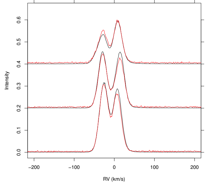
Fig. 6. Examples of H\beta (red) and H\alpha (black) lines from pure-sky fibers using UVES. A vertical shift was applied to spectra from different sky positions. The H\beta lines were scaled up by a factor of 7.
