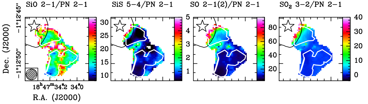
Fig. 4. Maps of integrated intensity ratios. The plots show the ratio between the PN integrated intensity and that of, from left to right, SiO J = 2-1 , SiS J = 5-4 , SO J = 2-1(2) , and SO 2 J_{Ka,Kb} = 3_{1,3} - 2_{0,2} . We show only the emission included in or close to the two PN-emitting regions 1 and 2, as the PN integrated emission goes rapidly to zero elsewhere. The star in the top left corner indicates the phase centre, and the ellipse in the bottom left corner in the first panel is the GUAPOS synthesised beam. The black and white contours correspond to the 3 mm continuum emission and the PN integrated emission, respectively, as shown in Fig. 1.
