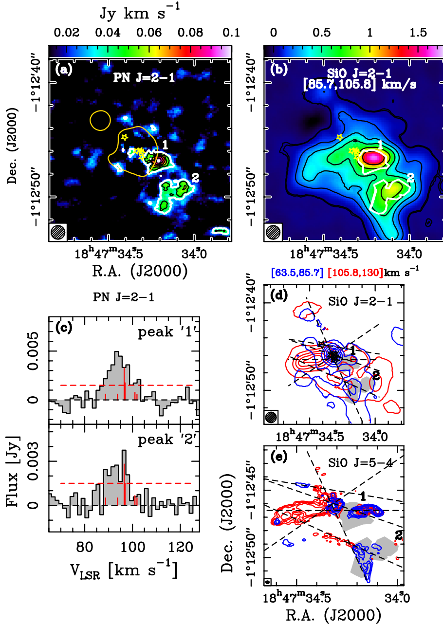
Fig. 1. Intensity maps of PN and SiO integrated in velocity. (a) PN J = 2-1 integrated in the range 85.7–105.8 \text{km s}^{-1} . The white contour is the 3\sigma rms level of the integrated map ( \sigma = 1.14 \times 10^{-2} \text{ Jy km s}^{-1} ), while the black contours are in steps of 1\sigma rms. The numbered regions 1 and 2 are those used to extract the spectra of all species analysed. The synthesised beam is in the bottom-left corner. The yellow contour is the 3 mm continuum emission at 16 mJy \text{beam}^{-1} , corresponding to 20\sigma rms. The yellow stars indicate the continuum sources identified by Beltrán et al. (2021). (b) Map of the intensity of SiO J = 2-1 integrated in the same velocity range as PN (colour scale). The PN emission regions identified in panel a are highlighted in white. Contours start at the 3\sigma rms level of the integrated emission ( 3 \times 10^{-2} \text{ Jy km s}^{-1} ), and correspond to 3, 15, 30, 50, 80, and 120\sigma . (c) Spectra of PN J = 2-1 extracted from the emission peak in regions 1 (upper panel) and 2 (lower panel). The red dashed horizontal line indicates the 3\sigma rms level, and the vertical lines show the position in velocity of the line hyperfine components. (d) SiO J = 2-1 emission integrated in the velocity ranges 63.5–85.7 \text{km s}^{-1} (blue contours) and 105.8–130.0 \text{km s}^{-1} (red contours). In both cases, the starting contour is the 3\sigma rms level of the integrated map ( 1.95 \times 10^{-2} \text{ Jy km s}^{-1} for the red contours, 1.62 \times 10^{-2} \text{ Jy km s}^{-1} for the blue contours), and the step is 25\sigma . The dashed lines correspond to the six outflows identified by Beltrán et al. (2022) from SiO J = 5-4 . The grey filled areas correspond to the PN emission regions 1 and 2 identified in panel a. (e) Same as panel d but for SiO J = 5-4 , obtained at an angular resolution of \sim 0.22'' with ALMA, and already published in Beltrán et al. (2018). The integration velocity intervals are the same as in panel d.
