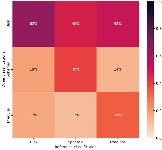
Figure 13. Matrix highlighting the level of agreement between the three classifiers for all galaxies with a disk or spheroid or those with irregular features. Overall, classifiers regularly agree when a galaxy has a disk, agree less often about galaxies with a spheroid, and are more likely to disagree about irregular features.
