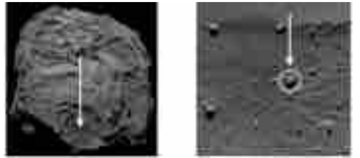
Fig. 6. Boulder-like feature in the Hatmehit region. The center of this feature is the first of two additional secondary features for the zero-longitude definition of the Cheops reference frame. Context image ( left ): subset of NAC_2014-08-06T01.19.14.554Z_ID20_1397549200_F22. Close-up ( right ): subset of NAC_2014-08-26T04.42.54.592Z_ID20_1397549500_F22.
