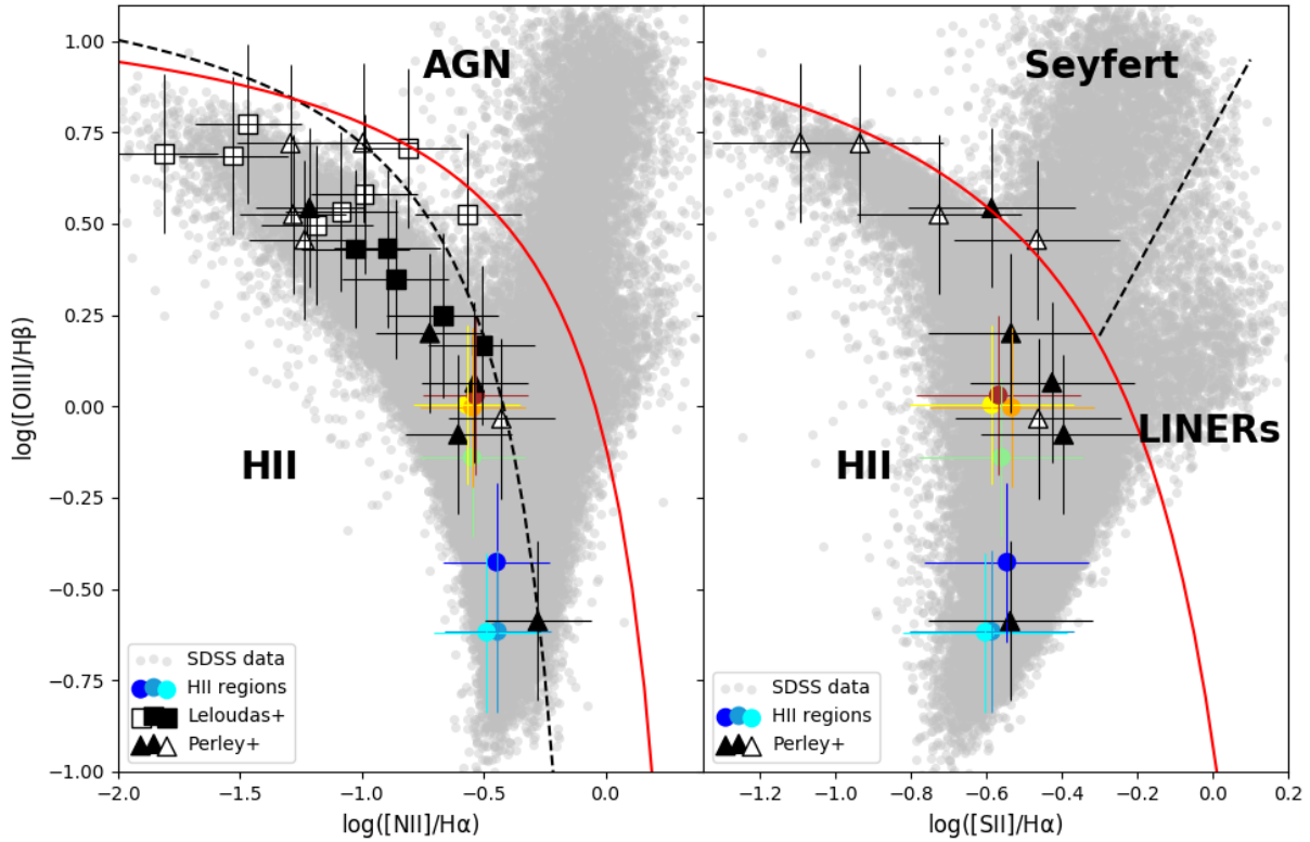
Fig. 5. BPT emission-line diagnostic used to distinguish the ionisation mechanism acting in the nebular gas in galaxies. Two distinct diagnostics are used here: [\text{O III}] \ 5008 \text{ \AA}/\text{H}\beta versus [\text{N II}] \ 6584 \text{ \AA}/\text{H}\alpha ( left ) and the [\text{S II}] \ 6718/32 \text{ \AA} doublet instead of [\text{N II}] ( right ). The solid red curves in both panels denote the theoretical demarcation line between AGNs and star-forming galaxies proposed by Kewley et al. (2001). In the left panel , the black dashed curve corresponds to the empirical demarcation between AGNs and SF galaxies proposed by Kauffmann et al. (2003), while in the right panel the black dashed line marks the division between active Seyfert galaxies and LINERs proposed by (Kewley et al. 2006). Grey data points are taken from the SDSS DR7 sample of galaxies described in Tremonti et al. (2004). Coloured circles correspond to the H II regions described in the text with the same colour-coding used in Fig. 1. Squares and triangles represent SLSN-host data from Leloudas et al. (2015) and Perley et al. (2016); empty symbols represent H-poor SLSNe, filled symbols H-rich SLSNe. The SLSN 2017egm location (light green circle) shows it is one of the most metal-rich Type I SLSN.
