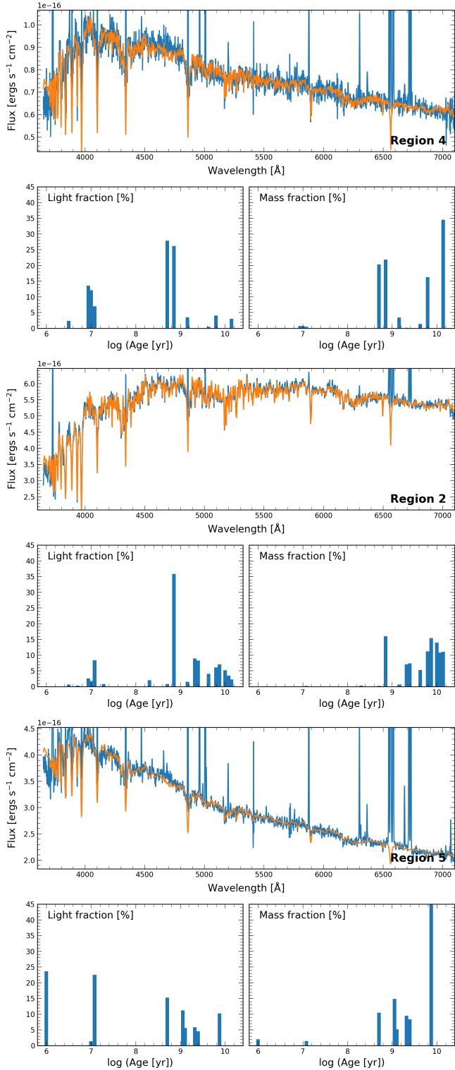
Fig. 10. From top to bottom, the stellar population analysis of H II regions 4 (the SLSN region), 2 (the galaxy centre), and 5 (the most active region in the galaxy). The upper panels show the fit to the observed spectral energy distributions, while the lower panels show the fraction in luminosity of stellar populations with different ages ( left ) and their contribution to the total stellar mass ( right ).
