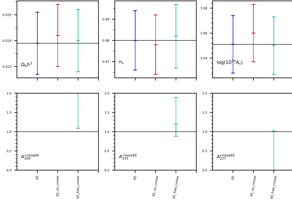
Fig. 87. Similar to Fig. 86 (but now for the Plik EE likelihood on the data), we explore the impact on the cosmological parameter posteriors of the empirical correlated-noise correction. We compare here the baseline analysis (correction included) with the cases where the correction is ignored or its amplitude is left to vary.
