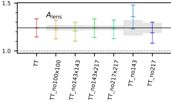
Fig. 83. Marginal means and 68% error bars for the A_L consistency parameter for \text{PlikTT} combined with Commander and SimAll EE , when removing either a single cross-spectrum, or all cross-spectra within a given frequency channel from the high- \ell part of the likelihood (i.e., Plik ). Grey bars represent the variance with respect to the full-frequency case, computed using Eq. (61).
