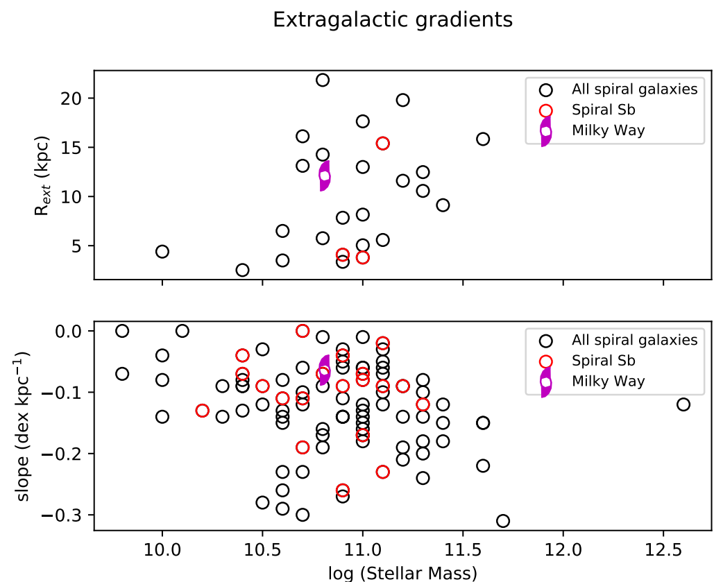
Figure 9. The figure shows the R_{\text{ext}} , the galactocentric radius at which the change of slope occurs, and the slope of the gradient in a sample of 95 spiral galaxies observed with MUSE@VLT in Sánchez-Menguiano et al. [172]. Colours and symbols are described in the legend.
