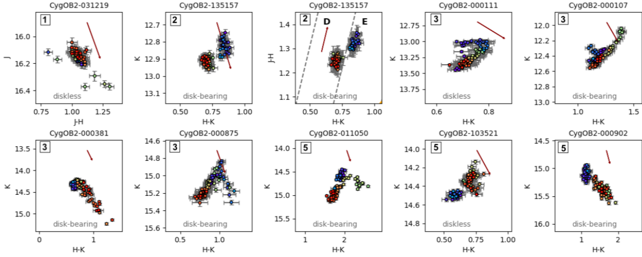
Fig. 13. Examples of stars with a compound behavior are shown inside color-color diagrams or color-magnitude diagrams. 1- Asymmetry with a distinct color; 2- Variable IR-excess; 3- Changing slope; 5- Mix of 2 and 3. Dark red arrows show the effect of interstellar reddening for A_V = 1 mag. The color of each data point reflects its observational date following the color-bar in Fig. 4.
