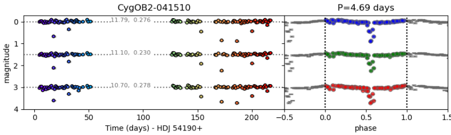
Fig. 18. Eclipsing binary candidate CygOB2-041510 (Fig. 8). Left: J, H, and K light curves for the star. The median magnitude and ptp amplitude are written in the plot, and the colors reflect the date of the observation, as in Fig. 4. Right: phased light curve for each band, folded using the detected period attributed to the occultation feature. J, H and K bands are shown as blue, green, and red respectively.
