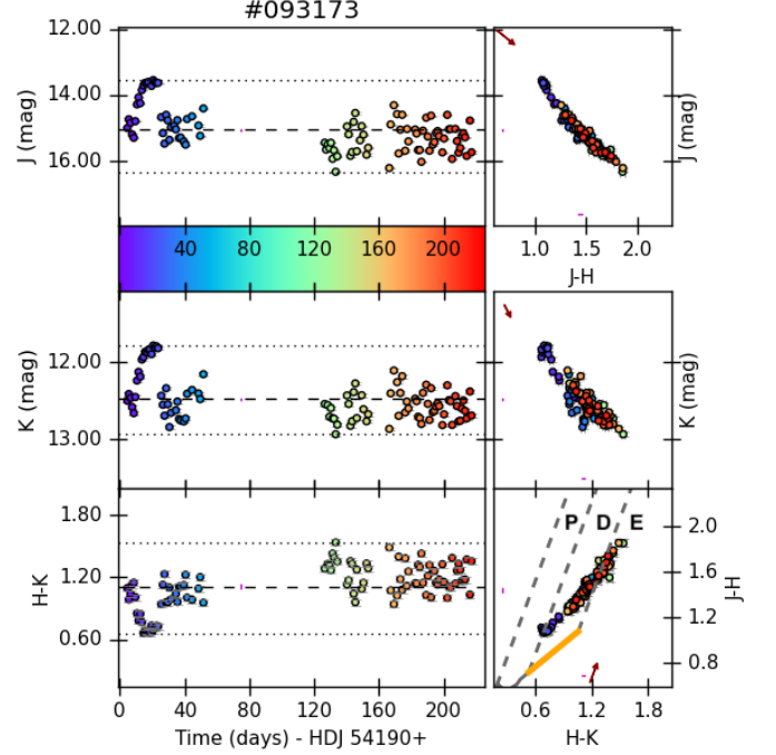
Fig. 4. Star CygOB2-093173 is a disk-bearing (Class II) star and an example of non periodic variable star, with S = 15.64 , and that presents reddening linear trajectories in the color-color and color-magnitude diagrams. Left , from top to bottom : J light curve, a color bar showing the color attributed for each observation date, K light curve, and H-K color curve. The dotted lines show maximum and minimum values in each light curves, and dashed lines show the median values. Right , from top to bottom : J vs. J-H color-magnitude diagram, K vs. H-K color-magnitude diagram, and color-color diagram with P, D, and E regions (discussed in Sec. 2). The dark red arrows show the effect of an interstellar reddening of A_V = 2^m . The vertical and horizontal magenta line segments show the median error in each axis. In each plot, error bars are shown in gray. When visible and close to the position of the star, a gray curve shows a Kraus & Hillenbrand (2007) empirical isochrone in the color-color diagram, and the orange line shows the T Tauri Locus. Each diagram has a range of 5\sigma around the median color or magnitude for that star.
