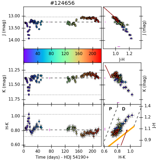
Fig. 7. Disk-bearing (Class II) star CygOB2-124656 is an example of an occultation variable that presents reddening linear trajectories in the color-color and color-magnitude diagrams. The star has S=3.59 and ptp amplitude of 0.43 and 0.17 in the J and K bands. The plots, colors, and symbols are the same as in Fig. 4.
