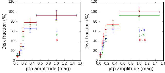
Fig. 3. Disk fraction as a function of peak to peak amplitude for each near-IR band (left) and color (right). In both plots, circles show the center of each ptp amplitude bin and horizontal bars indicate the size of each bin. Vertical bars show the standard errors of a Poisson counting in that bin.
