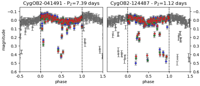
Fig. 17. Phased light curve for each band, folded using the secondary detected period found for the eclipsing binary candidates presented in Fig. 16. J, H and K bands are shown as blue, green, and red respectively.
