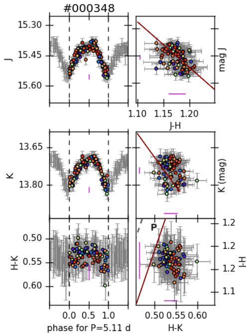
Fig. 5. Star CygOB2-000348 is an example of a diskless periodic variable, with S=1.62 , a ptp amplitude of 0.13 and 0.11 mag in the J and K bands respectively, and that does not show periodicity in color. The plots, colors, and symbols are the same as in Fig. 4, but with the light curves and color curve phased with the period of the star, P=5.11 d.
