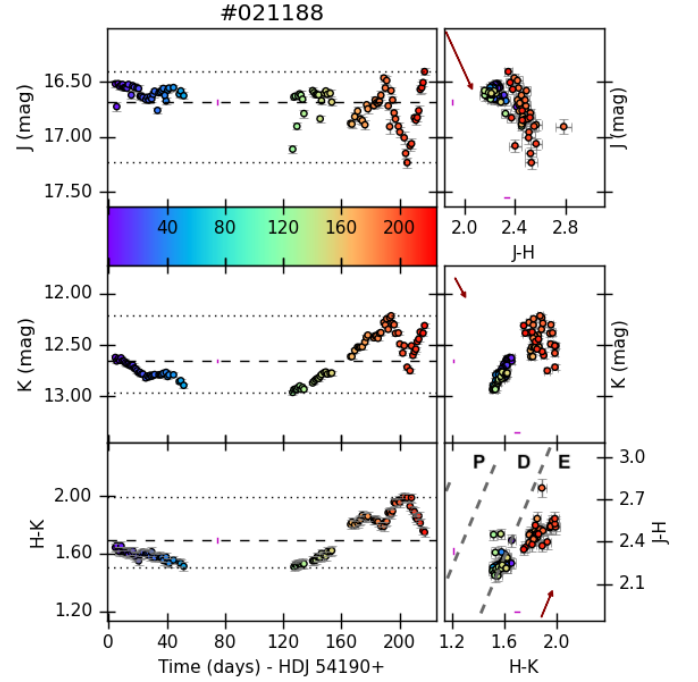
Fig. 12. Disk-bearing (Class II) star CygOB2-021188 ( S=1.0 ) is an example of compound variability showing a variable near-IR excess and a changing slope during the observed time. The plots, colors, and symbols are the same as in Fig. 4.
