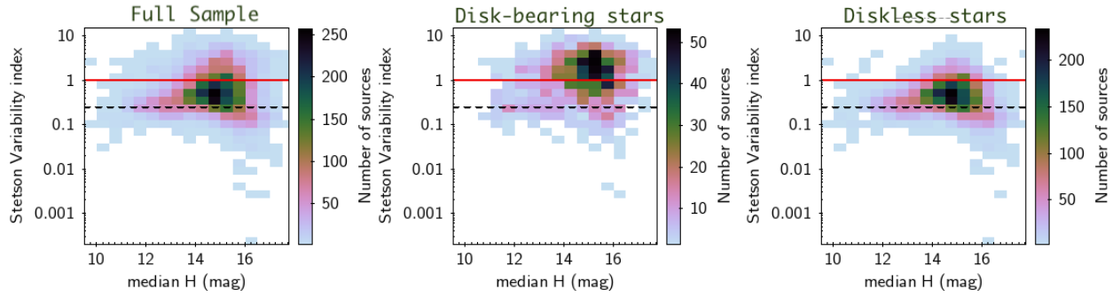
Fig. 2. Distribution of Stetson variability index as a function of H median magnitude for the full sample of candidate members (left), disk-bearing stars (middle), and diskless stars (right). The red line shows S = 1 , and the dashed black line shows S = 0.25 .
