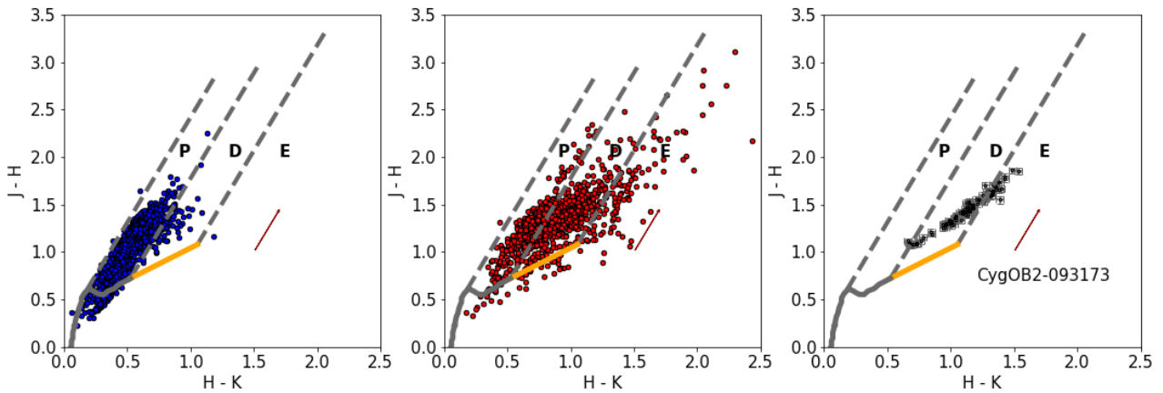
Fig. 1. Near-IR (JHK) color-color diagrams. Left and middle panels show the median colors of the 3811 diskless stars (blue dots) and the 1272 disk-bearing stars (red dots) analyzed in the present study. Right panel: shows the CygOB2-093173 variable star. Black dots show the color of the star in each observed night. The regions labeled as “P”, “D” and “E” are the regions typically occupied by stars with normal photospheric colors, disk-bearing colors, and extreme near-IR excess respectively. The dark red arrow shows the effect of the interstellar reddening for the median visual extinction expected for stars in the CygOB2 association ( A_V = 4.1^m ). The gray solid curve shows an empirical dwarf sequence by Kraus & Hillenbrand (2007) and the orange line shows the Meyer et al. (1997) T Tauri locus. Dashed gray lines show extinction paths of A_V = 10^m for 0.6 M_\odot and 0.08 M_\odot stars, and the truncation point of the T Tauri locus.
