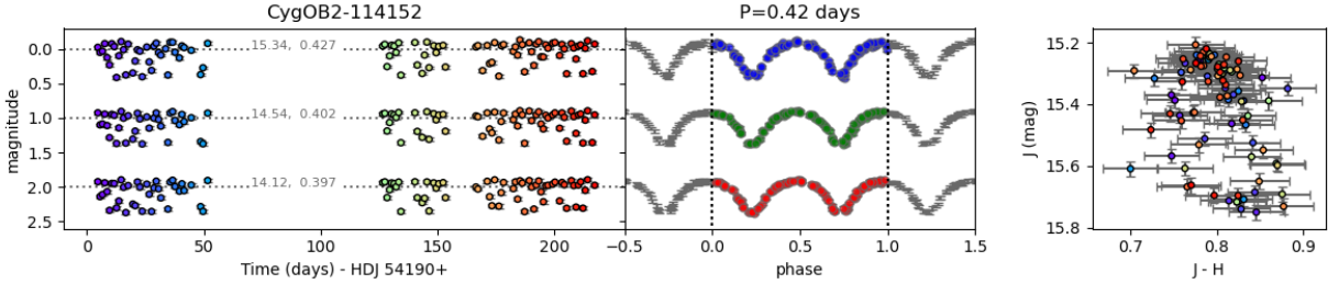
Fig. 21. Star CygOB2-114152 is a periodic candidate and compound in this survey but it is reported as an eclipsing binary in HSP11. Left: J, H, and K light curve. The median magnitude and ptp amplitudes are written in the plot, and the colors reflect the date of the observation, as in Fig. 4. Middle: phased light curve for each band. J, H and K bands are shown as blue, green, and red respectively. The period reported by HSP11 (below our detection limit) was adopted in the phased light curve. Right: J vs. J-H CMD. Colors reflect the date of the observation, as in Fig. 4.
