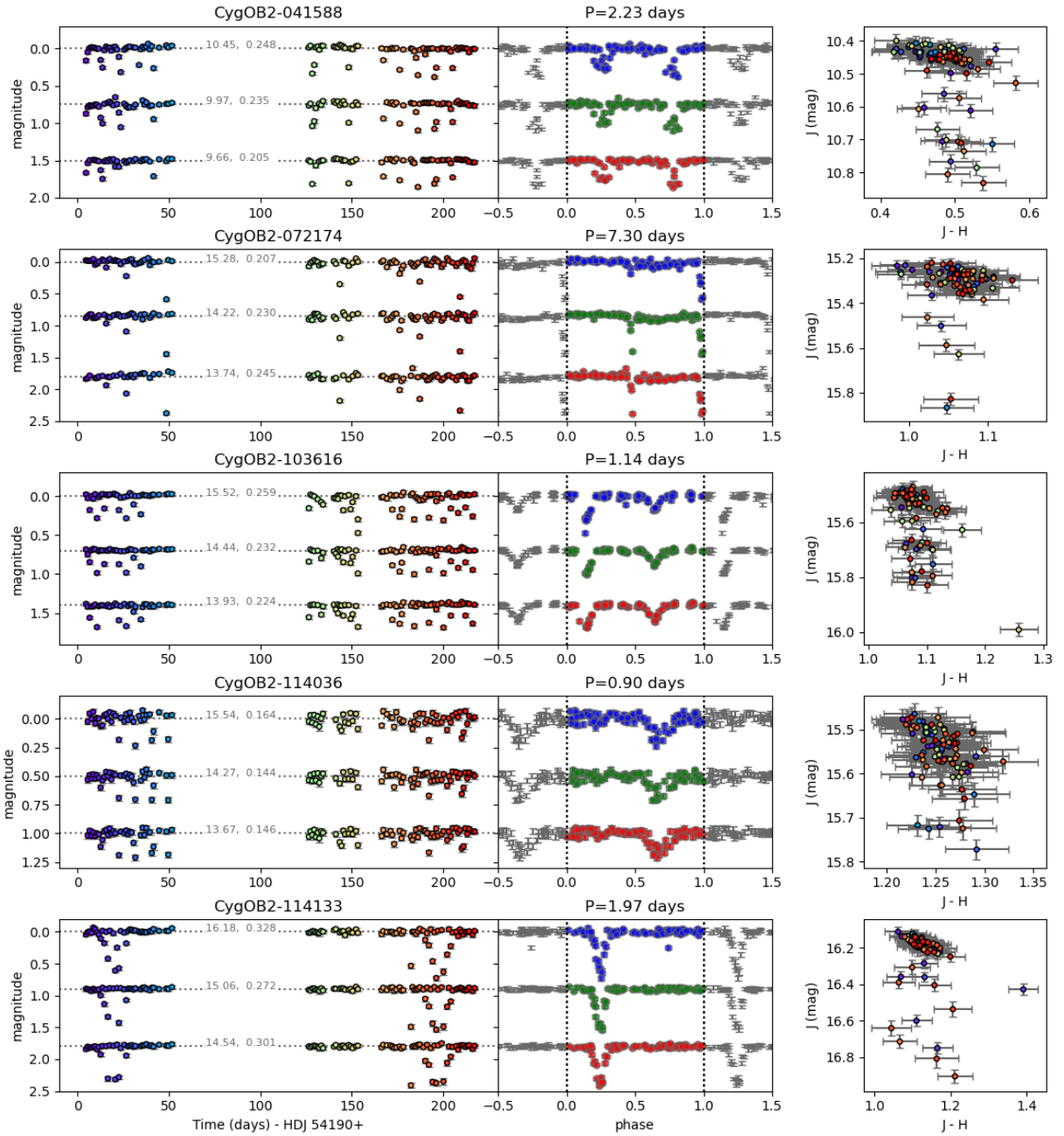
Fig. 19. Five periodic eclipsing binary candidates. Left: J, H, and K light curves for each star. The median magnitude and ptp amplitude are written in the plot, and the colors reflect the date of the observation, as in Fig. 4. Middle: phased light curve for each band, folded using the detected period attributed to the occultation feature. J, H and K bands are shown as blue, green, and red respectively. Right: J vs. J-H CMD. Colors reflect the date of the observation, as in Fig. 4.
