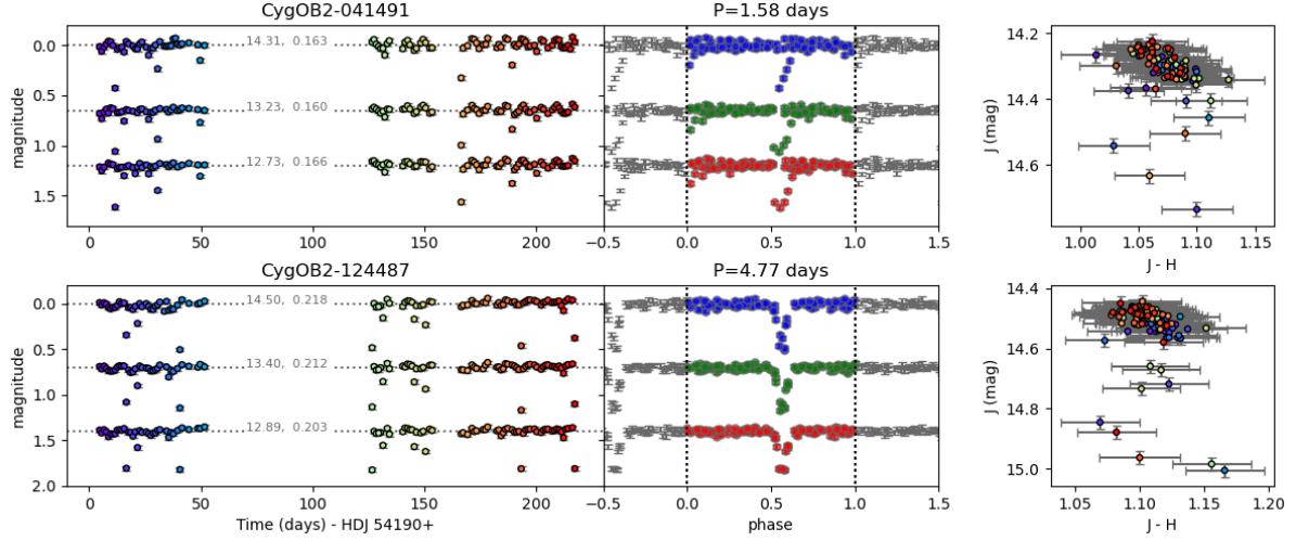
Fig. 16. Two multiperiodic eclipsing binary candidates. Left: J, H, and K light curves for each star. The median magnitude and ptp amplitude are written in the plot, and the colors reflect the date of the observation, as in Fig. 4. Middle: phased light curve for each band, folded using the detected period attributed to the occultation feature. J, H and K bands are shown as blue, green, and red respectively. Fig. 17 shows the folded light curves for the secondary period. Right: J vs. J-H CMD. Colors reflect the date of the observation, as in Fig. 4.
