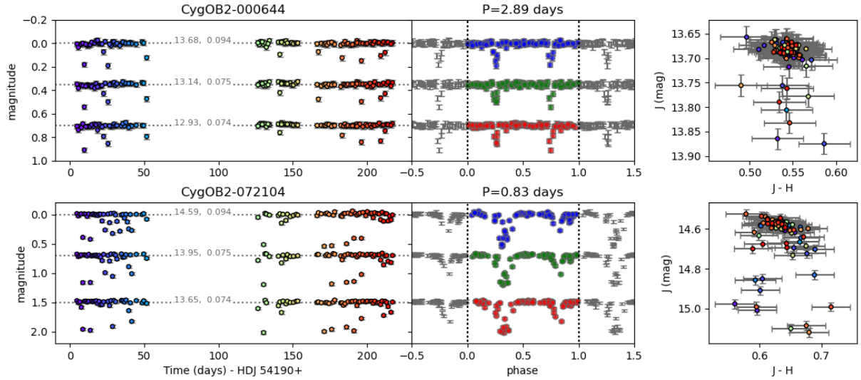
Fig. 20. Stars CygOB2-000644 and CygOB2-072104 are both occultation and compound variables and were considered as eclipsing binary candidates in the present study. They are also reported as eclipsing binaries in HSP11. Left: J, H, and K light curves for each star. The median magnitude and ptp amplitude are also written in the plot, and the colors reflect the date of the observation, as in Fig. 4. Middle: phased light curve for each band. J, H and K bands are shown as blue, green, and red respectively. Right: J vs. J-H CMD for the same star. Colors also reflect the date of the observation, as in Fig. 4.
