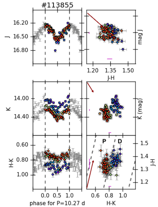
Fig. 6. Star CygOB2-113855 is an example of a disk-bearing (Class II) periodic star. With S=2.77 and ptp amplitude of 0.31 and 0.36 mag in the J and K bands, the star is also periodic in color. It is also an example of a compound variable with a variable IR-excess. The plots, colors, and symbols are the same as in Fig. 4, but with the light curves and color-curve phased with the period of the star, P=10.3 d.
