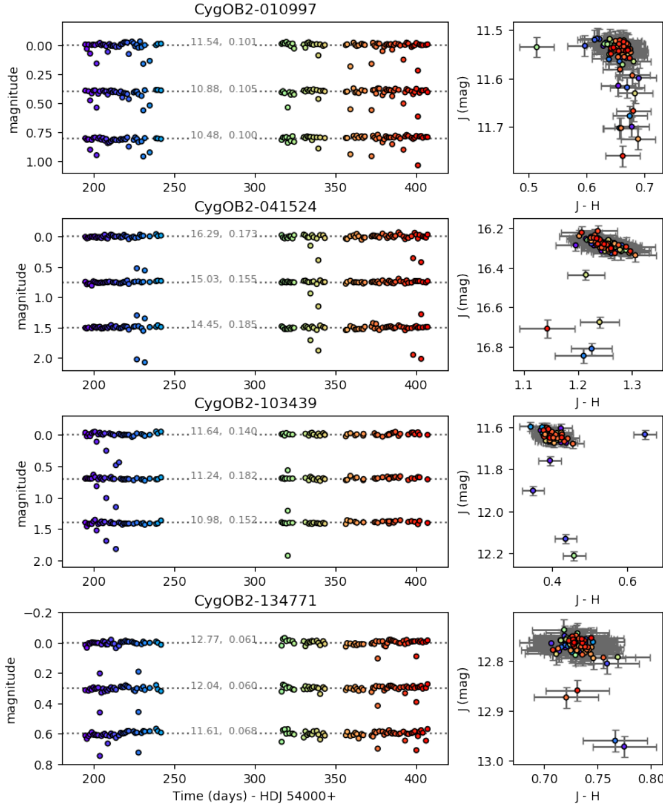
Fig. 15. Four eclipsing binary candidates that were not periodic in our study. Left: J, H, and K light curves for each star. The median magnitude and ptp amplitude are written in the plot. Right: J vs. J-H CMDs. In both left and right plots, colors reflect the date of the observation as in Fig. 4.
