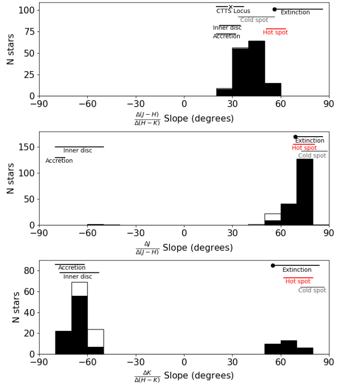
Fig. 14. Distribution of slopes measured in the color-color and color-magnitude diagrams. The figure shows slopes for J-H vs. H-K (top), J vs. J-H (middle), and K vs. H-K (bottom) diagrams. We plotted the expected slopes for each physical mechanism as line segments, following the ranges in Table 7. The X mark shows the exact position of the T Tauri Locus. The black circle shows the slope expected for the typical dust opacity index in the ISM. Black bars show the stars in S_1 sample and with precision in the light curve better than 5%, empty bars show stars in the S_2 sample or with precision worse than 5%.
