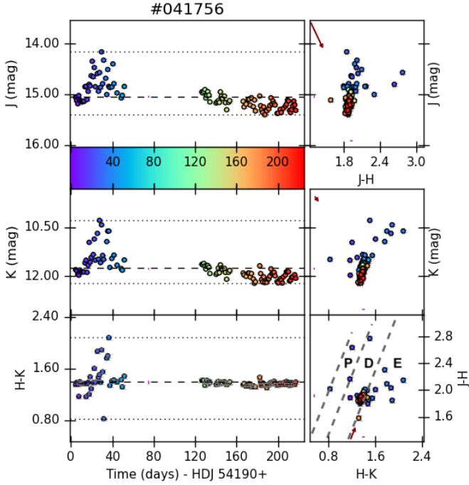
Fig. 11. Disk-bearing (Class II) star CygOB2-041756 ( S=10.4 ) is an example of a mixed variable with a long term variability mixed with burst features in the first epochs observed. The star is a compound variable with asymmetries in the light curve having a distinct color behavior. The plots, colors, and symbols are the same as in Fig. 4.
