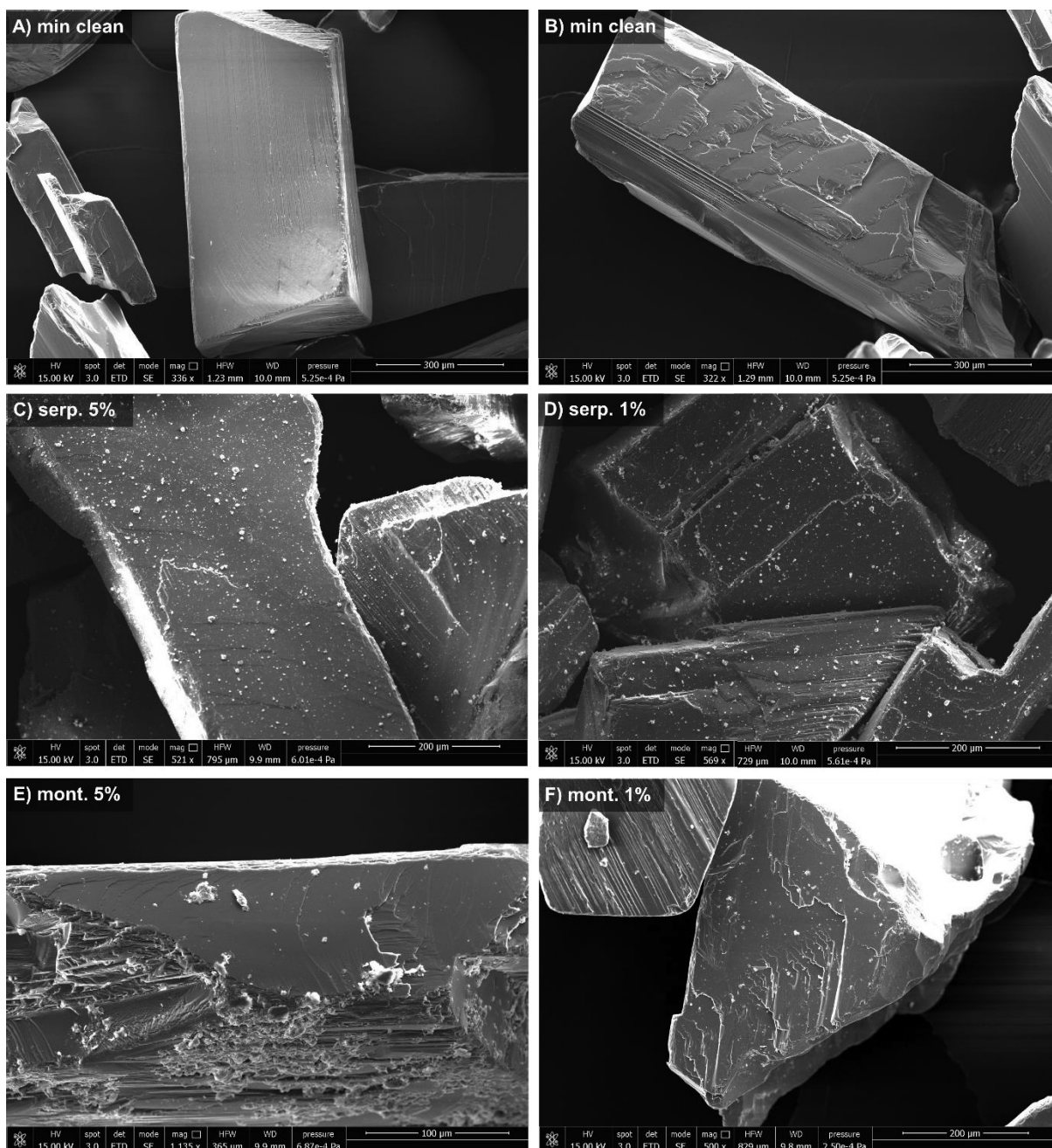
Figure S4 Secondary electrons SEM image of enstatite sample before (panel A and B) and after mixing with 5% and 1% of serpentine (panel C and D) and montmorillonite (panel E and F). As visible in the images of the mixed samples the hyperfine hydrated component tends to stick on the flat surface of the bigger grain size anhydrous component.
