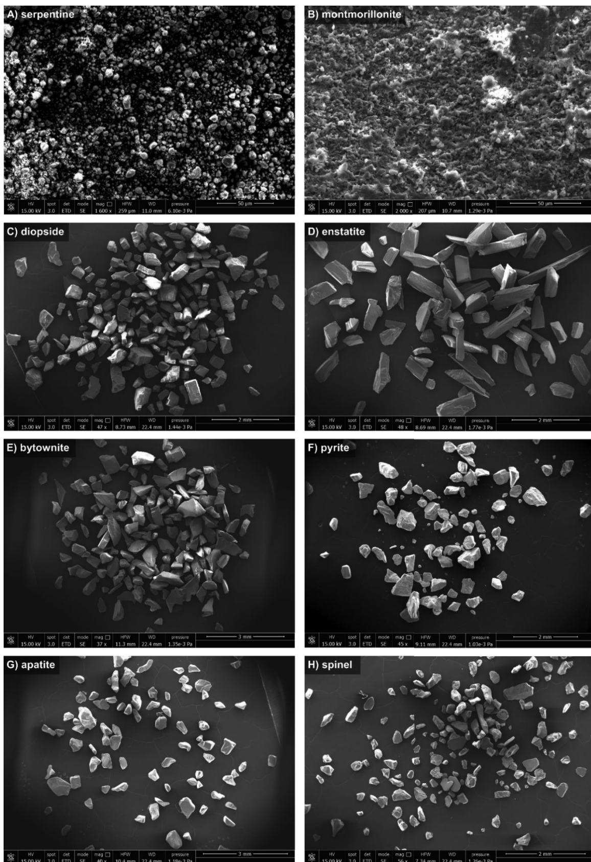
Figure 1 Secondary electrons SEM images of the mineral samples used to produce the mix. Image order: (A) serpentine, (B) montmorillonite, (C) diopside, (D) enstatite, (E) bytownite, (F) pyrite, (G) apatite and (H) spinel. The scalebar at the bottom left of each pictures varies from 50 µm (for
