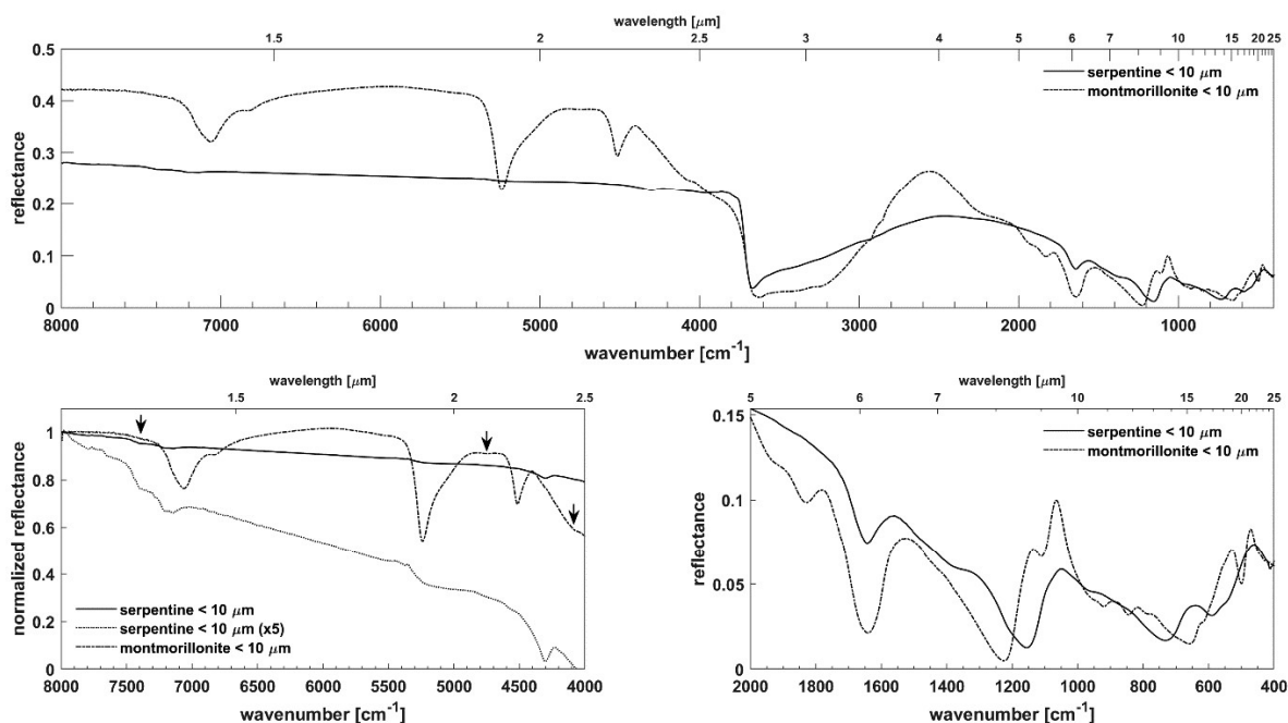
Figure S1 Infrared spectrum of serpentine (solid line) and montmorillonite (dash-dot line). Top panel, full range of acquisition. Bottom left panel, detail of normalized reflectance in the NIR region 8000-4000 cm -1 (1.25-2.5 μm) with serpentine spectrum shown in original and with x5 magnitude to enhance the presence of minor bands (dotted line). Black arrows are showing position of very faint features in montmorillonite spectrum. Bottom right panel, detail of MIR region 2000-400 cm -1 (5-25 μm).
