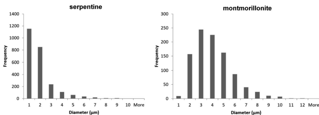
Figure S2 Grain size distribution in the serpentine sample (left) and montmorillonite sample (right) from SEM analysis
