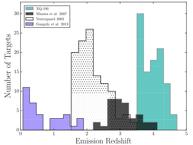
Figure 1. Redshift distribution of our quasar sample (diagonal filled histogram), compared with previous works: Vestergaard (2003, open dotted histogram), Misawa et al. (2007, dark shaded histogram) and Ganguly et al. (2013, diamond filled histogram). XQ-100 enlarge the studied redshift range to higher values.
