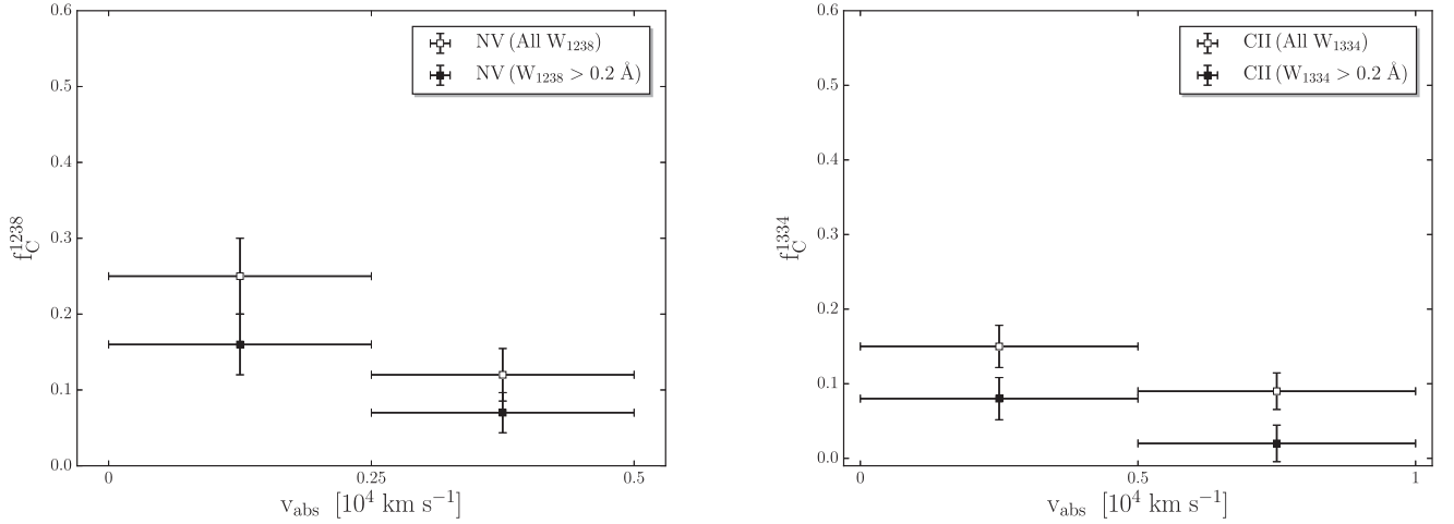
Figure 9. Covering fractions, f_C , for \text{N V}_{1238} (left) and \text{C II}_{1334} (right) estimated from the fraction of quasars exhibiting at least one absorber with W_0 > 0.2 \text{ Å} (filled circles) or for the whole sample (open circles), in bins of velocity offset from z_{\text{em}} .
