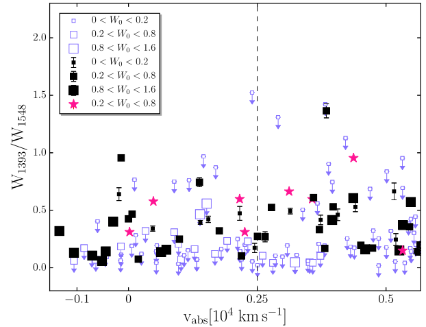
Figure 10. Velocity offset distribution with respect to the quasar z_{\text{em}} of the N v and C iv (left), Si iv and C iv (right) equivalent width ratio. The size of the symbol represents the corresponding W_{1548} Å strength, indicated by the legends. Detections ( 3\sigma ) are the filled squares. The open squares show the rest-frame equivalent width 3\sigma upper limit values for the non-detections. The DLA systems present in our sample are marked by open stars (filled stars) in the left-hand panel (right-hand panel) and they show N v upper limits (Si iv detections). The vertical dashed lines represent the separation of the velocity range in two bins.
