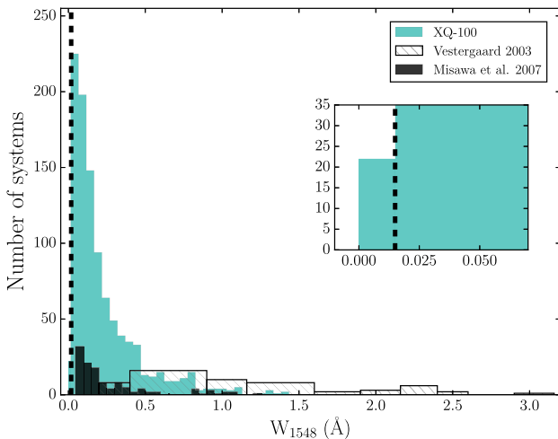
Figure 3. The rest-frame equivalent width distribution of all C IV systems in our sample (light-shaded histogram). The vertical dashed line marks our detection limit of 0.015 \text{ Å} . Distributions measured by previous works are also shown: Vestergaard (2003, diagonal filled histogram) and Misawa et al. (2007, dark shaded histogram). The insert shows the details of the bottom-left region of the histogram.
