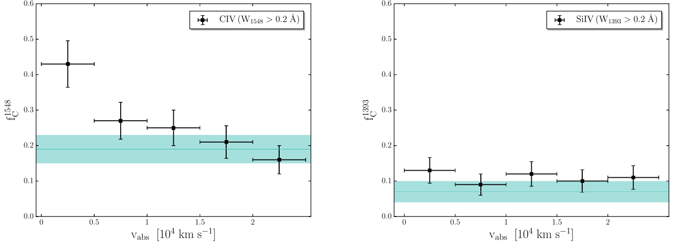
Figure 8. Covering fractions, f_C , for \text{C IV}_{1548} (left) and \text{Si IV}_{1393} (right) estimated from the fraction of quasars exhibiting at least one absorber with W_0 > 0.2 \text{ Å} , in bins of velocity offset from z_{\text{em}} (horizontal error bars). The horizontal solid line in both plots shows the mean covering fraction for W_0 > 0.2 \text{ Å} lines measured for random 5000 \text{ km s}^{-1} intervals far from the quasars, the shaded band represents the 1\sigma error.
