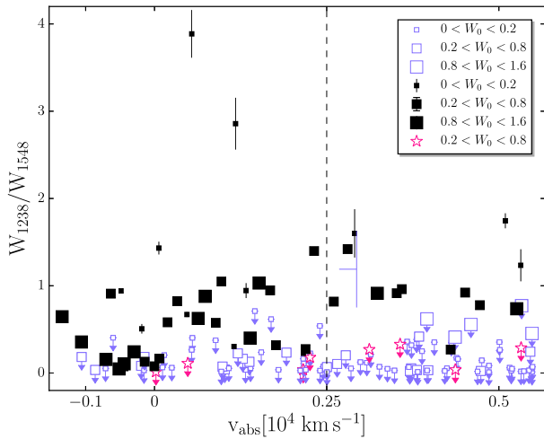
Figure 10. Velocity offset distribution with respect to the quasar z_{\text{em}} of the N v and C iv (left), Si iv and C iv (right) equivalent width ratio. The size of the symbol represents the corresponding W_{1548} Å strength, indicated by the legends. Detections ( 3\sigma ) are the filled squares. The open squares show the rest-frame equivalent width 3\sigma upper limit values for the non-detections. The DLA systems present in our sample are marked by open stars (filled stars) in the left-hand panel (right-hand panel) and they show N v upper limits (Si iv detections). The vertical dashed lines represent the separation of the velocity range in two bins.
