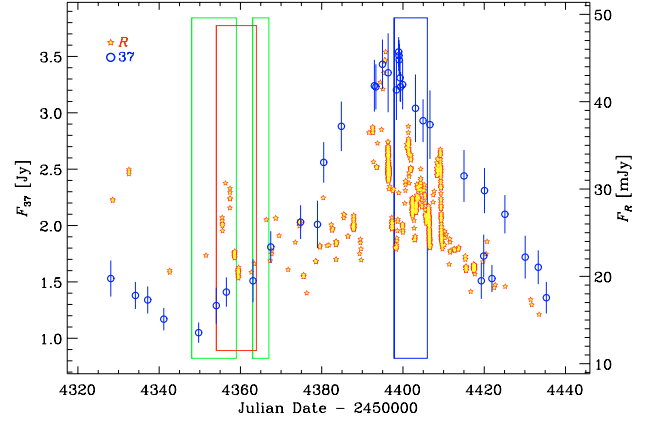
Fig. 4. 37 GHz light curve of 0716+714 in August–November 2007 (blue circles) compared to the R -band flux densities in the same period (red, yellow-filled stars), rescaled to have the optical and radio maxima at the same level.
