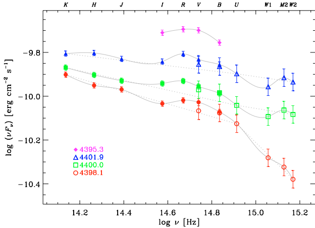
Fig. 5. Spectral energy distributions (SEDs) of 0716+714 in late October 2007, constructed with W2 M2 W1 U B V data from Swift-UVOT (empty symbols) and ground-based GASP-WEBT BVR IJHK data (filled symbols). The numbers in the legend refer to the Julian Dates of the observations. The dotted lines connect the K , U , and W2 data; together with the cubic splines through the spectra, they help to better distinguish the main features of the SEDs (see text).
