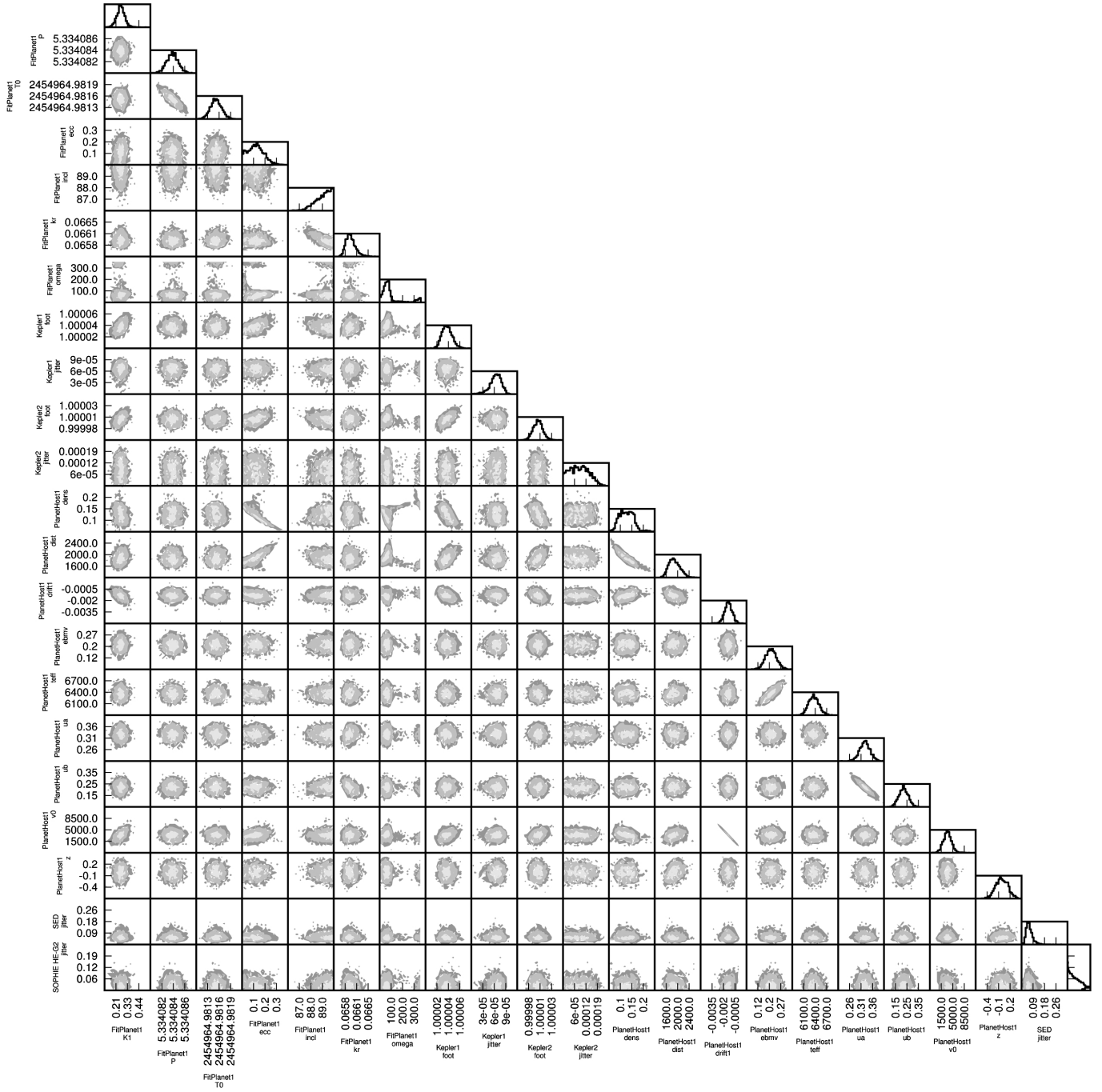
Fig. 12. Two-parameter joint posterior distributions of the MCMC jump parameters of the fit with stellar models of KOI-206. The 39.3%, 86.5%, and 98.9% joint confidence regions are denoted by three different gray levels. The histogram of each parameter is shown at the top of each column, except for the parameter on the last line that is shown at the end of the line.
