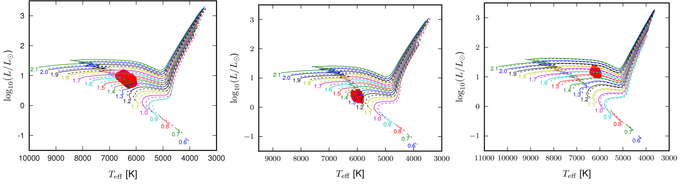
Fig. 4. Stellar evolution tracks from STAREVOL , from the zero-age main-sequence stage to 25 Gyr age, in the luminosity-effective temperature plane for [\text{Fe}/\text{H}] = 0.00, 0.25 , and -0.20 (from left to right, solid line) and [\text{Fe}/\text{H}] = 0.10, 0.35 , and -0.15 (from left to right, dashed line) with the joint posterior distributions of the MCMC (98.9% joint confidence region is denoted in red) for KOI-206, KOI-614, and KOI-680, respectively. The mass in solar masses is annotated at the beginning of the main sequence of each track.
