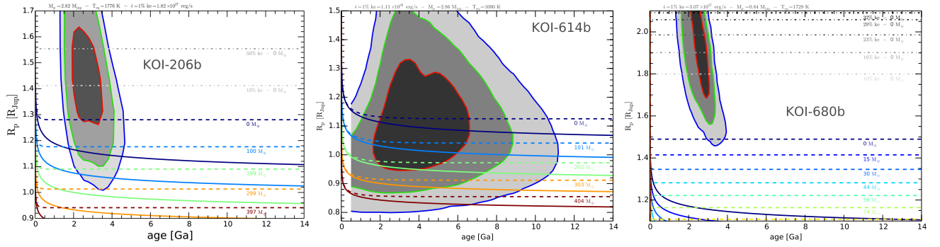
Fig. 6. Evolution of the planet radius as a function of the age. KOI-206b with mass 2.82 M_{Jup} and effective temperature 1776 K is plotted to the left, KOI-614b ( 2.86 M_{Jup} and 1000 K) in the center plot, and KOI-680b ( 0.84 M_{Jup} and 1729 K) in the right plot. The 68.3%, 95.5%, and 99.7% joint confidence regions are denoted by black, dark gray, and light gray areas, respectively. The curves represent the thermal evolution of a respective planet mass and equilibrium temperature. Text labels indicate the amount of heavy elements in the planet (its core mass in Earth masses). Dashed lines represent planetary evolution models for which 0.25% of the incoming stellar flux ( \epsilon ) is dissipated into the core of the planet, whereas plain lines do not account for this dissipation (standard models). Dashed-dotted lines (gray shades) are coreless models with higher amounts of dissipated energy, as labeled.
