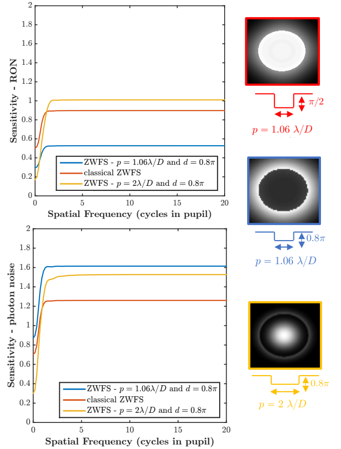
Fig. 4. Sensitivities to RON and photon noise for a different configuration of the ZWFS. The “dark” ZWFS configuration corresponds to p = 1.06\lambda/D and d = 0.8\pi .
