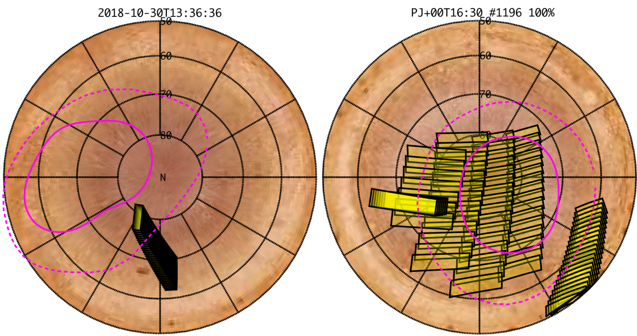
Figure 1: Simulation with JSPT (JIRAM Software Planning Tool), coverage of the North Pole with filter M . The overlapped yellow strips represent the predicted FOVs.
