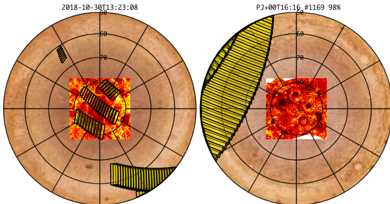
Figure 2: Simulation with JSPT. Coverage of the North Pole with filter L.
