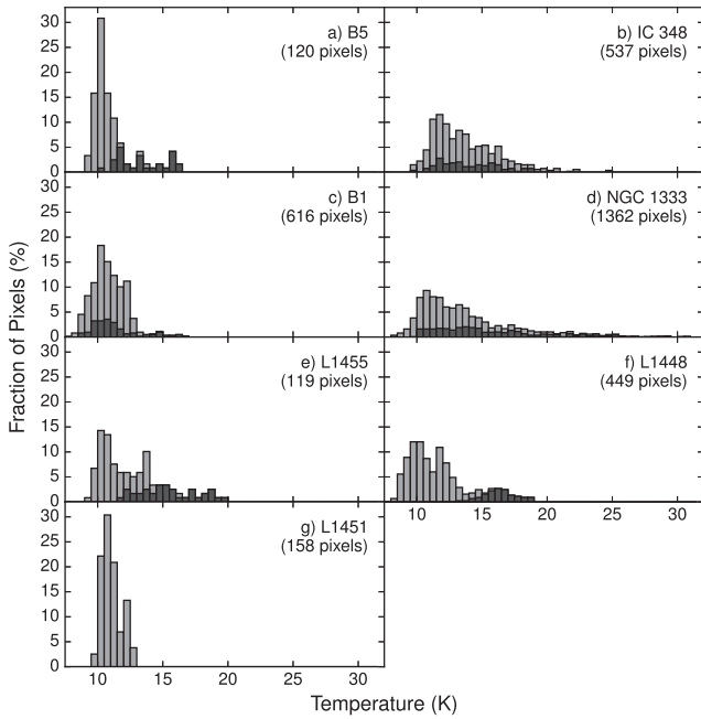
Figure 4. Histograms of derived T_d values in the seven Perseus clumps. All the pixels within a clump are shown in light gray while the pixels within a 72''.6 diameter (i.e., two Herschel 500 \mu\text{m} beam widths) centered on a Class 0/I and Flat YSOs are shown in dark gray.
