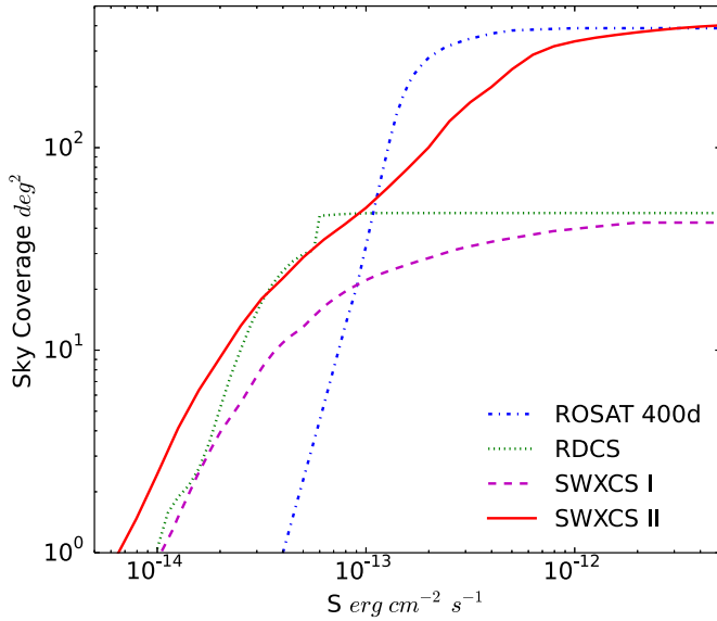
Figure 4. Sky coverage of SWXCS as a function of the soft band flux (solid line). For comparison, we also show the sky coverage of the first release of the SWXCS (Paper I, dashed line), of the ROSAT 400d catalog (Burenin et al. 2007, dot-dashed line), and of the RDCS (Rosati et al. 1998, dotted line).
