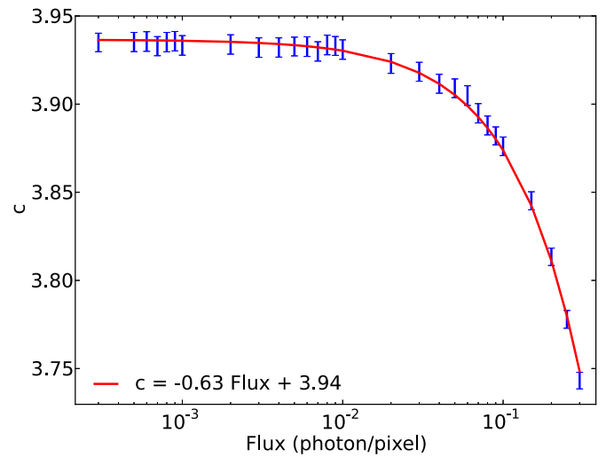
Figure 13. Correlation between the best-fit c parameter in Equation (A2) and the input background. The red line is the best-fit Equation (A3).
