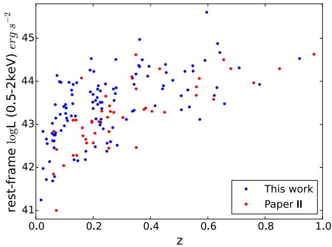
Figure 10. Restframe 0.5–2 keV luminosity vs. redshift. More accurate luminosities measured with X-ray spectroscopy in Paper II are used when available (red points).
