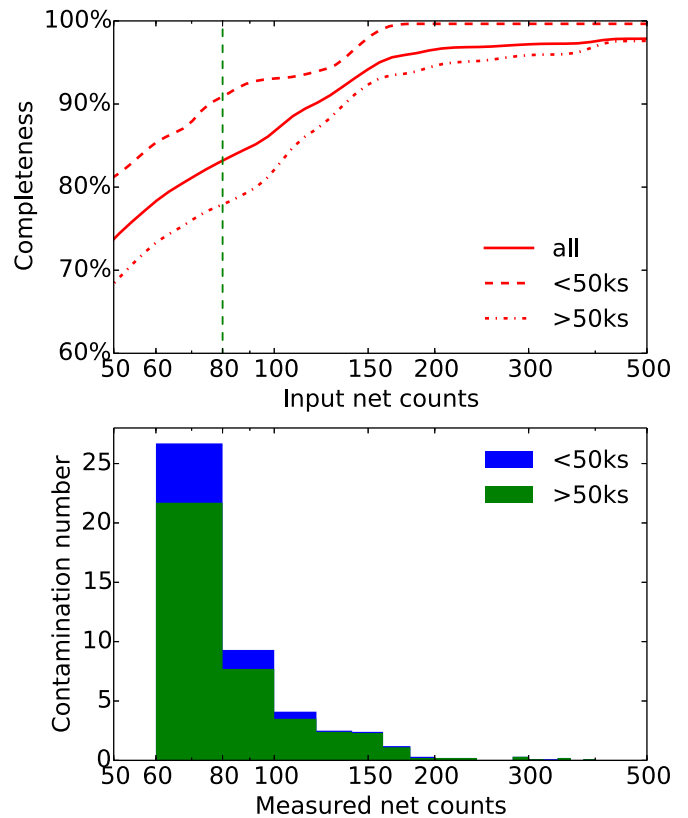
Figure 3. Upper panel: solid red line shows the completeness of SWXCS (defined as the ratio of recovered sources and the number of input sources) as a function of the input net counts as measured with our simulations. The dashed red lines indicate the completeness obtained only considering those fields with an exposure of less than 50 ks (long dashed line) and larger than 50 ks (dot dashed line). Lower panel: histogram of the number of spurious sources expected in the entire SWXCS catalog from our simulations in bins of net detected counts. The different colors show the number of spurious sources found in fields with exposure times above (green shaded area) and below (blue shaded area) 50 ks.
