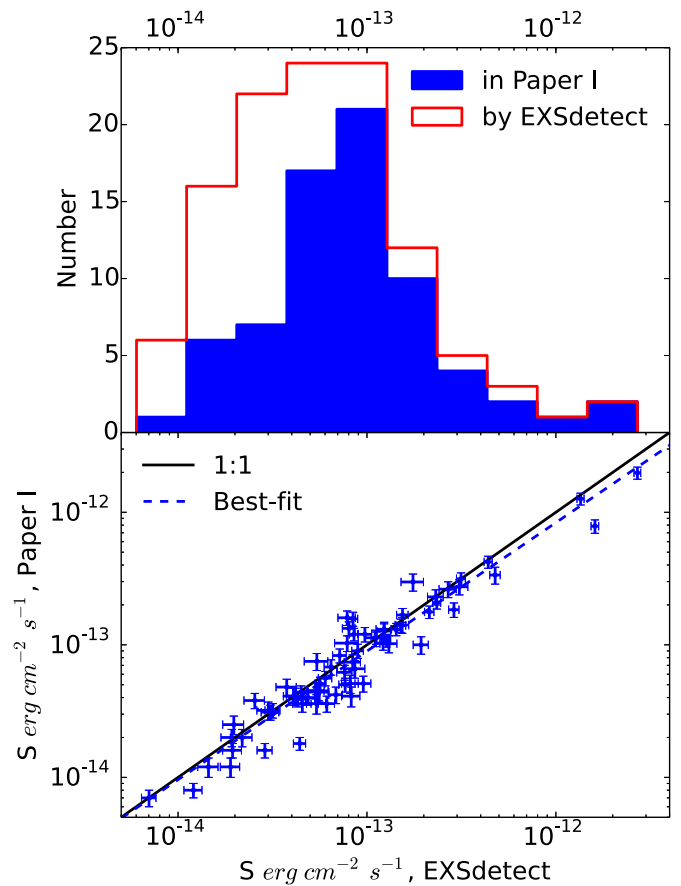
Figure 7. Upper panel: histogram distributions of the EXSdetect -measured soft-band fluxes of all the sources detected with EXSdetect in the same GRB fields used in Paper I (red histogram) and of the 71 SWXCS sources already presented in Paper I (blue filled histogram). Lower panel: for the 71 SWXCS sources that Paper I has in common, the soft-band fluxes S_{\text{Paper I}} measured in Paper I within R_{\text{ext}} , compared with the soft-band fluxes S_{\text{EXS}} measured in this paper with EXSdetect from a source region defined by the VT+FOF algorithm. Black solid line shows the relation S_{\text{Paper I}} = S_{\text{EXS}} , while the blue dashed line shows the best fit \log(S_{\text{Paper I}}/10^{-13}) = 0.97 \times \log(S_{\text{EXS}}/10^{-13}) - 0.05 .
