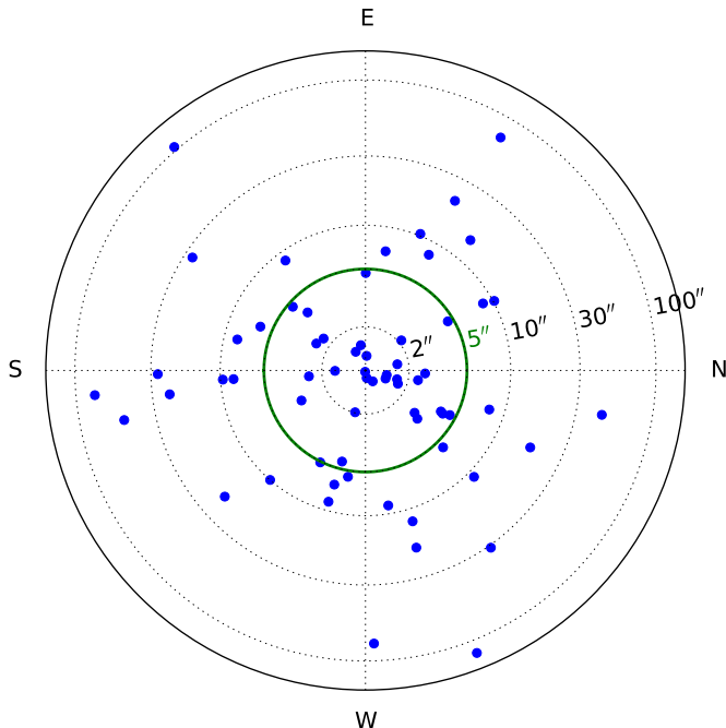
Figure 9. Displacements between the source positions in Paper I and the positions found in this work in units of arcseconds. The green circle shows the median separation corresponding to 5''.
