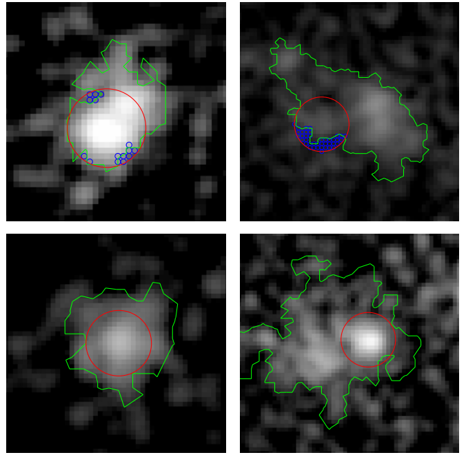
Figure 16. Four examples of disambiguations in real XRT images. Red circles mark the position of the candidate extended source, and have a radius of 7 pixels. Green lines enclose the FOF regions that reach the same flux level as the PSF at a radius of 7 pixels. Blue circles mark pixels outside the FOF regions but inside the red circles. The two sources in the upper panels are classified as unresolved, while the sources in the lower panels are classified as extended.
