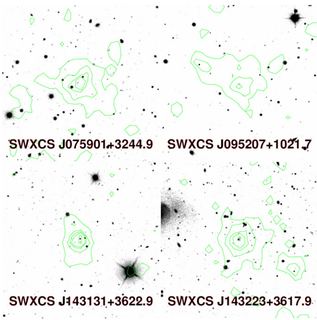
Figure 12. SDSS r -band images of four SWXCS sources with soft-band fluxes less than 5 \times 10^{-14} \text{ erg cm}^{-2} \text{ s}^{-1} and without obvious optical counterparts. These sources are among the high- z cluster candidates in the SWXCS. The image sizes are 5' \times 5' . The X-ray contour generating method is the same as used in Figure 11.
