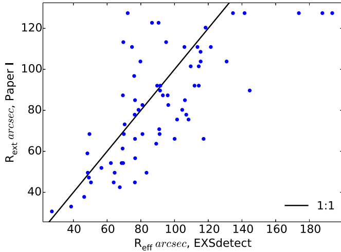
Figure 8. Extraction radius R_{\text{ext}} used in Paper I to define the source region, compared to the effective radius R_{\text{eff}} for EXSdetect sources. The solid line shows the relation R_{\text{ext}} = R_{\text{eff}} .
