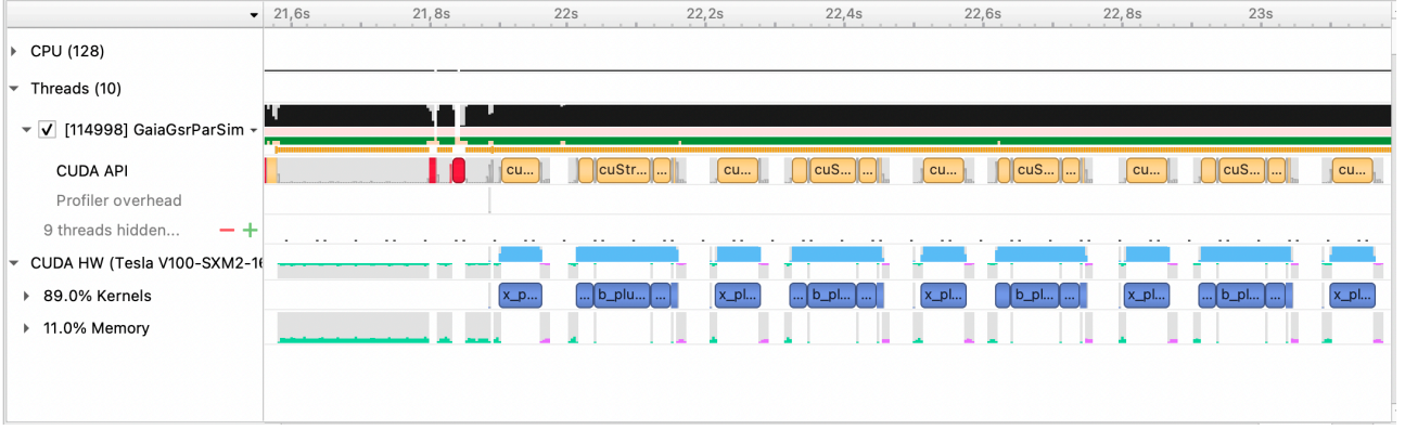
Figure 5: Output of the NVIDIA Nsight Systems profiler [14] for a run of the MPI+OpenACC code with 4 iterations of the LSQR algorithm. The code is parallelized on 4 MPI processes on one node of Marconi100, and thus on 4 GPUs, and the system occupies a memory of 10 GB. This output shows the portion of the OpenACC code from line 4 to line 17 of Figure 3.
