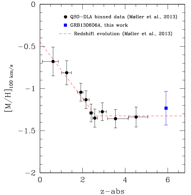
Fig. 6. Results from Møller et al. (2013) with the high-redshift measurement of GRB 130606A included. [\text{M}/\text{H}]_{100 \text{ km s}^{-1}} is the metallicity expected for DLAs with \Delta V = 100 \text{ km s}^{-1} , based on the overall mass-metallicity relation. The data of Møller et al. (2013; filled circles) favour a break in the evolution of the mass-metallicity relation at z \sim 2.6 (dashed line), which is also supported by our measurement of GRB 130606A (filled square). We assumed for this point \Delta V = 90 \text{ km s}^{-1} and [\text{M}/\text{H}] = -1.3 \pm 0.2 ; see text.
