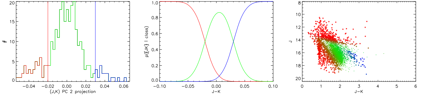
Figure D2. Same as Figure 1, but for the second PC of \{J, K\} . Additionally, during the classification (right panel), the higher of the foreground likelihoods between the first (Figure D1) and second components is chosen.
