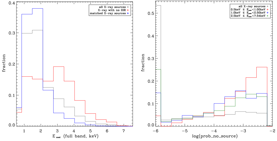
Figure C1. Left: distributions of the median energy of the detected photons for all the X-ray sources detected in our survey (gray), for those matched with OIR counterparts (blue), and for the X-ray sources without an OIR counterpart (red). Right: distribution of the ACIS Extract parameter prob-no-source for the X-ray sources with no OIR counterpart separated according to their median photon energies, with soft (0.5–1 keV; red), medium (1–2.5 keV; blue), hard (2.5–7.5 keV; green), and all (black).
