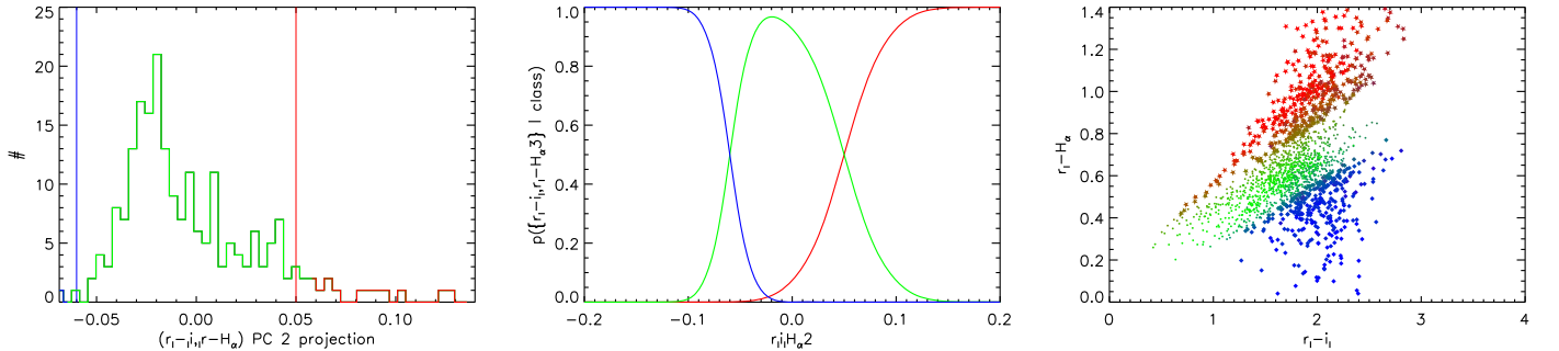
Figure D4. Same as Figure 1, but for the second PC of \{r_I - i_I, r_I - H\alpha\} .
