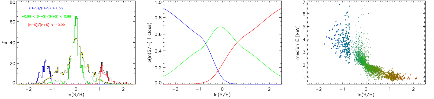
Figure 3. Likelihood generation for X-ray colors. Left: histogram of X-ray colors filtered on hardness ratios for a well-measured subsample, with the histogram for the full sample shown as the dashed black/yellow line normalized to the same number of objects and overplotted. Middle: the likelihoods generated by square-root transformation of the Gaussian components, with the tails modified to be linearly decreasing. Right: class assignments with points color coded as RGB tuples as in Figure 1.
