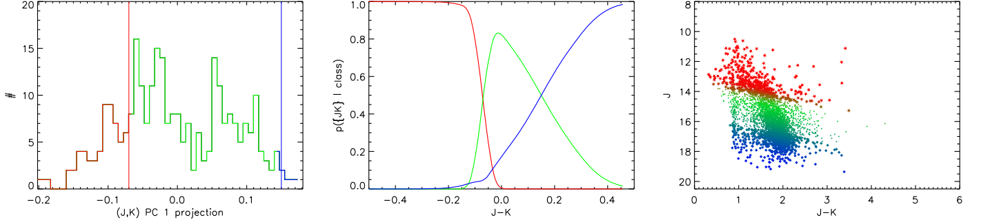
Figure D1. Same as Figure 1, but for the first PC of \{J, K\} .
