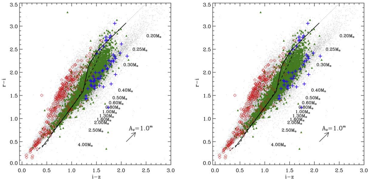
Figure 6. r-i vs. i-z diagrams of all the sources with good OSIRIS or SDSS photometry. The solid line is the 2.5 Myr isochrone from Siess et al. (2000) after applying the F96 transformation between the UBVR I and the u_i g_i r_i i_z z_i photometric systems, and the dashed line is from the MIST database. The extinction vector is obtained from O’Donnell (1994). The corresponding masses are indicated with a horizontal displacement from the isochrone. The classifications are according to the automated NBC method (left) and after manual reclassification (right) and show foreground objects (red diamonds), members (green circles), and background objects (blue crosses).
