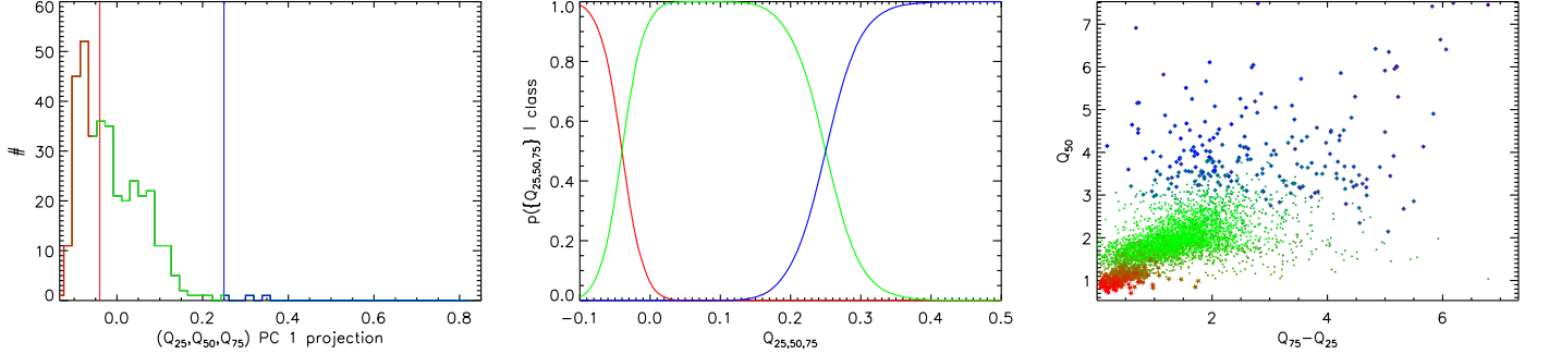
Figure D6. Same as Figure 1, but for the first PC of \{Q_{25}, Q_{50}, Q_{75}\} .
