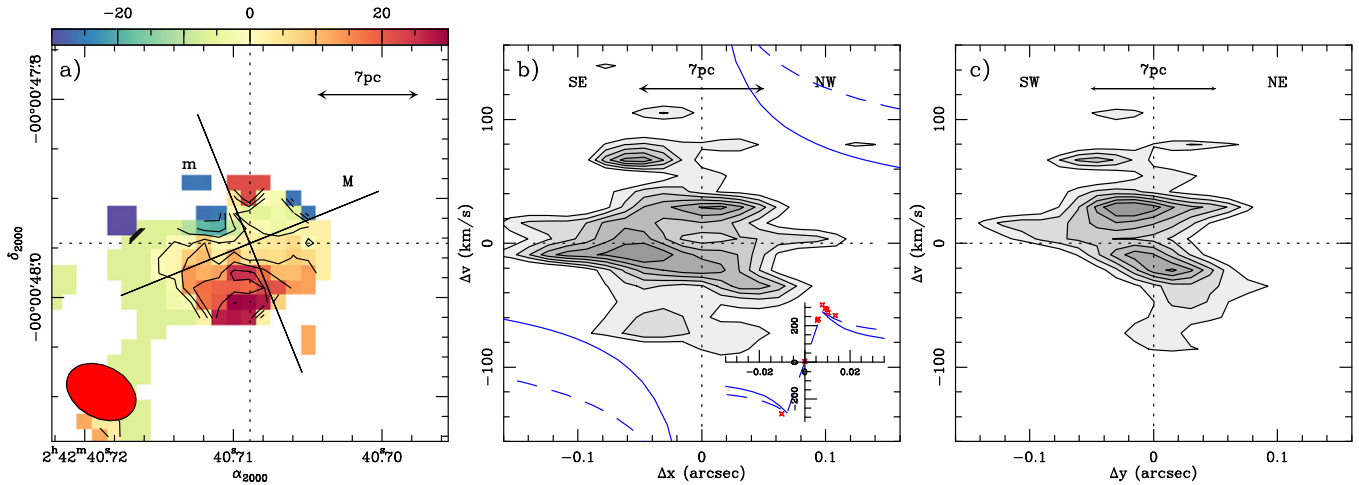
Figure 5. (a) CO(6–5) mean-velocity map of the torus. The contours span the range (-30 \text{ km s}^{-1} \text{ to } 30 \text{ km s}^{-1}) in steps of 10 \text{ km s}^{-1} . The black lines labeled as M and m show, respectively, the orientations of the major and minor axes of the CO torus ( PA^M = 112^\circ \pm 20^\circ , PA^m = 22^\circ \pm 5^\circ ). (b) CO(6–5) position–velocity diagram along the M axis. Contours go from 2\sigma to 7\sigma in steps of 1\sigma , where 1\sigma = 4 \text{ mJy}^{-1} \text{ beam}^{-1} . The inset shows the velocities relative to v_{\text{sys}} as a function of radius (in arcseconds) as derived for the \text{H}_2\text{O} megamaser spots (red markers) detected along PA^{\text{maser}} = 140^\circ \pm 5^\circ (GR96, GA01). The dashed (solid) blue curve shows the best-fit sub-Keplerian (Keplerian) rotation curve v_{\text{rot}} \propto r^{-\alpha} of GR96 with \alpha = 0.31 (0.50). (c) Same as middle panel, but for the m axis. In all panels, velocities refer to v_o(\text{HEL}) = 1136 \text{ km s}^{-1} and (\Delta x, \Delta y) —offsets are relative to the AGN position.
