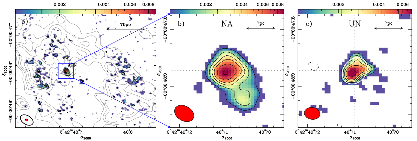
Figure 1. (a) Dust continuum emission at 694 GHz (432 \mu\text{m} ) mapped by ALMA in the CNL of NGC 1068. The natural (NA)-weighted map is shown in color scale (in \text{Jy beam}^{-1} -units) and (black) contour levels ( 3\sigma , 5\sigma , 7\sigma , 9\sigma , 12\sigma , and 16\sigma where 1\sigma = 0.5 \text{ mJy beam}^{-1} ). The red-filled ellipse in the bottom left corner represents the beam size at 694 GHz ( 0''.07 \times 0''.05 at PA = 60^\circ ). The gray contours (10%, 20%, 30% to 90% in steps of 20% of the peak value: 49 \text{ mJy beam}^{-1} ) identify the dust emission obtained in GB14 using ALMA with a lower resolution: 0''.4 \times 0''.2 at PA = 50^\circ (black ellipse). The dashed lines highlight the location of the AGN at (\alpha_{2000}, \delta_{2000}) = (02^{\text{h}}42^{\text{m}}40.709^{\text{s}}, -00^\circ00'47''.95) . (b) A close-up of the dust continuum emission shown in left panel. (c) The same as middle panel but using a uniform (UN)-weighted set of data with a spatial resolution: 0''.06 \times 0''.04 at PA = 82^\circ . Contour levels are 3\sigma , 4\sigma , 5\sigma , 6\sigma , and 8\sigma , where 1\sigma = 0.7 \text{ mJy beam}^{-1} . The white ellipse identifies the disk emission found by the task UV_FIT.
