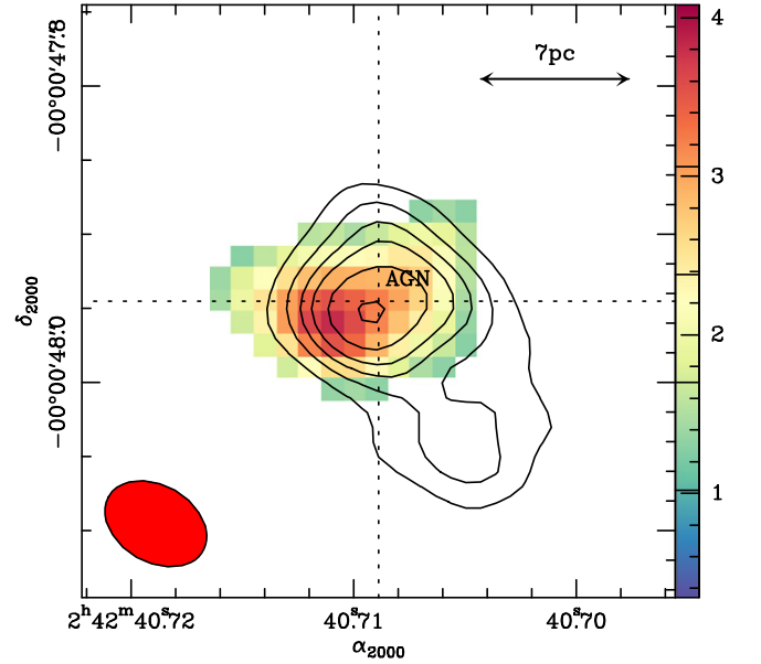
Figure 3. Overlay of the continuum emission contours of Figure 1 on the CO(6–5) emission (color scale) from the AGN torus. Units are in \text{Jy km s}^{-1} \text{ beam}^{-1} .
