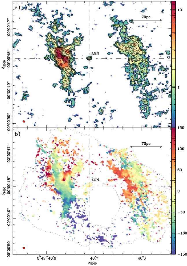
Figure 2. (a) The CO(6–5) intensity map of the CND of NGC 1068. The color scale and contours span the range: 3\sigma , 5\sigma , 9\sigma , 12\sigma , 15\sigma to 40\sigma in steps of 5\sigma , where 1\sigma = 0.34 \text{ Jy km s}^{-1} \text{ beam}^{-1} . The filled ellipse at the bottom left corner represents the CO(6–5) beam size ( 0''.07 \times 0''.05 at PA = 60^\circ ). (b) The CO(6–5) mean-velocity map (color scale). The dashed polygon identifies the region where significant ( >5\sigma ) emission was detected in GB14. Velocities refer to v_0(\text{HEL}) = 1136 \text{ km s}^{-1} .
