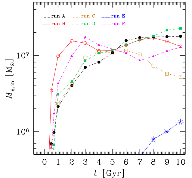
Fig. 2. Mass of the gas that lies in the inner 15 kpc of the S0 galaxy ( M_{\text{g, in}} ) for all simulations, as a function of time. Time t = 0 corresponds to the first periaapsis passage. Long-short dashed black line and filled black circles: run A; solid red line and open red circles: run B; dotted ochre line and open ochre squares: run C; dashed green line and filled green squares: run D; long-dash-dotted blue line and blue asterisks: run E; short-dash-dotted magenta line and filled magenta triangles: run F.
