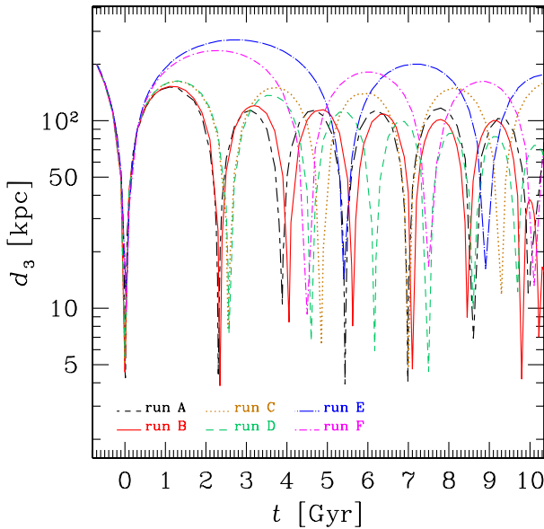
Fig. 1. Radial distance of the satellite galaxy from the centre of the primary galaxy for all simulations, as a function of time. Time t = 0 corresponds to the first periaapsis passage. Long-short dashed black line: run A; solid red line: run B; dotted ochre line: run C; dashed green line: run D; long-dash-dotted blue line: run E; short-dash-dotted magenta line: run F.
