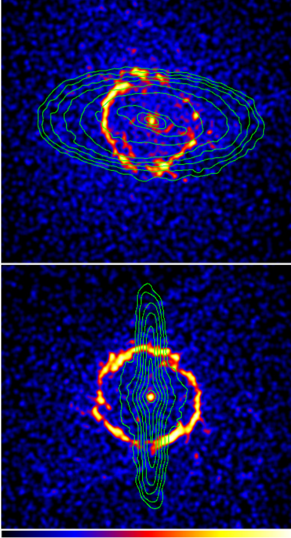
Fig. 5. Projected density of gas (logarithmic colour-coded map) and stars (isocontours) of the primary galaxy 4 Gyr after the first periaapsis passage. Top panel: run C. Bottom panel: run D. Each panel measures 79 \times 67 kpc.
