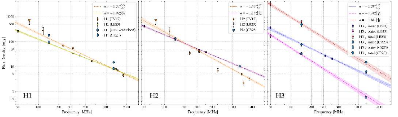
Fig. 7. Integrated spectral index measurements and fits for the three components: H1, H2 and H3, as presented in Table 2 and discussed in the text. Dashed/dotted/dot-dashed lines show the best-fit spectral index, with the shaded region denoting the 1\sigma uncertainty, coloured according to the extraction region in Figures 3. References ‘TV17’, ‘LB23’ and ‘CR23’ refer to Venturi et al. (2017), Bruno et al. (2023) and this work, respectively. Orange fits were performed solely on the measurements from Venturi et al. (2017), whereas the yellow and purple fits to H1 and H2, as well as all fits to H3, were performed using the combination of our new measurements plus those from Bruno et al. (2023). Note that the different sets of measurements for H1 were derived using different areas, as described in the text; the ‘CR23-matched’ measurements denote those derived using the same region as Bruno et al. (2023), whereas the ‘CR23’ measurement was derived over the more full extent of H1. When fitting to the data from Venturi et al. (2017), the 74 MHz measurement for H1 and H2 is an upper limit and was thus excluded from the initial fit. Likewise, the measurements at 234 MHz, 608 MHz, and 1377 MHz for H2 were derived from data with sparser uv -coverage, and were excluded from the fit. See Venturi et al. (2017) for further details.
