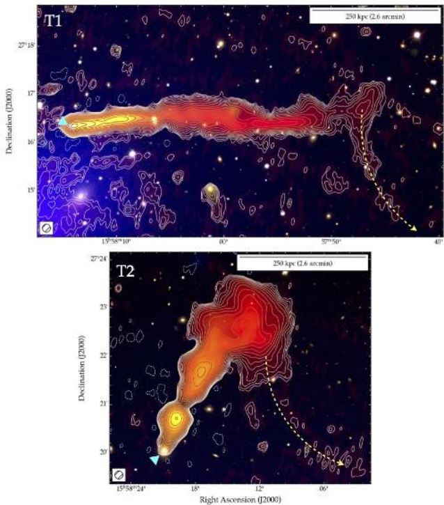
Fig. 5. Colour-composite images of the tailed radio galaxies T1 (top) and T2 (bottom) embedded in the ICM of Abell 2142, as per Figure 1. Contours denote the radio surface brightness measured by LOFAR at 143 MHz as per Figure 2. Cyan markers point to the host galaxies. Yellow curves indicate the direction of further faint ultra-steep spectrum emission that is only partially recovered at this resolution, which likely traces ancient fossil plasma from these radio galaxies.
