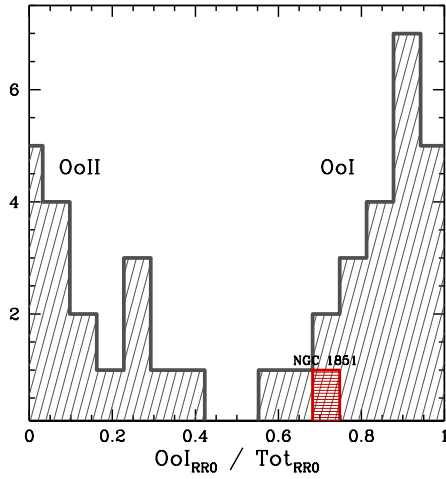
Fig. 2. A histogram of the ratio of OoI stars in the Milky Way GCs. The Oosterhoff ratio of the NGC 1851 RR0 Lyrae stars is highlighted.
