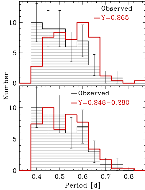
Fig. 3. Top: A comparison between the observed NGC 1851 RR Lyrae periods versus the theoretical periods with a constant Y=0.265 (Gratton et al. 2012). Bottom: The results when using a He abundance with minor helium variations ( Y \sim 0.248-0.280 ) versus the observed periods.
