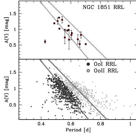
Fig. 1. Top: Period-amplitude diagram for our sample of RR0 Lyrae variables in NGC 1851. Bottom: Period-amplitude relation for 1097 RR0 Lyrae variables in 40 Galactic GCs. Our division of OoI and OoII-type RR Lyrae variables are shown by dark and light circles, respectively. The lines derived by Clement & Shelton (1999) for OoI and OoII RR0 are overplotted.
