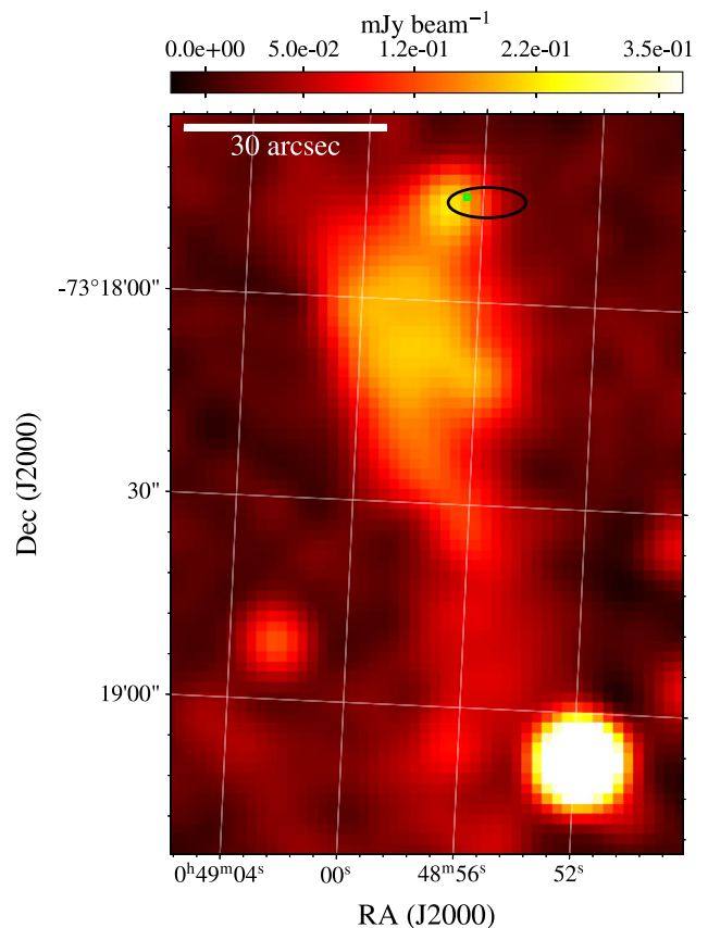
Figure 13. The PWN associated with PSR J0048–7317 from the Cotton et al. (2024) MeerKAT image of the SMC. The Paper I SEEKAT localization region is shown, with its 3\sigma error approximated to a black ellipse. The new radio timing position is shown as a green square, and firmly places the pulsar at the leading edge of the bow-shock nebula.
