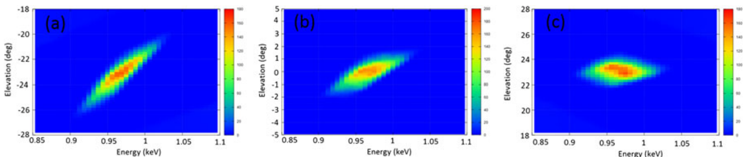
Figure 6. Response function calculated with SIMION showing the transmission rate over the energy and elevation response for three deflector potentials considered: (a) U_{\text{def}} = -170 V, (b) 0 V, and (c) 170 V. For this simulation both deflectors are polarized in an antisymmetrical fashion.
