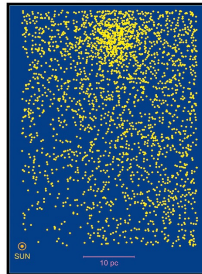
Gaia
