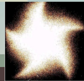
TNG 3.58m
