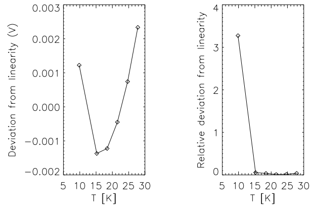
Figure 4.15: Deviation from linearity
