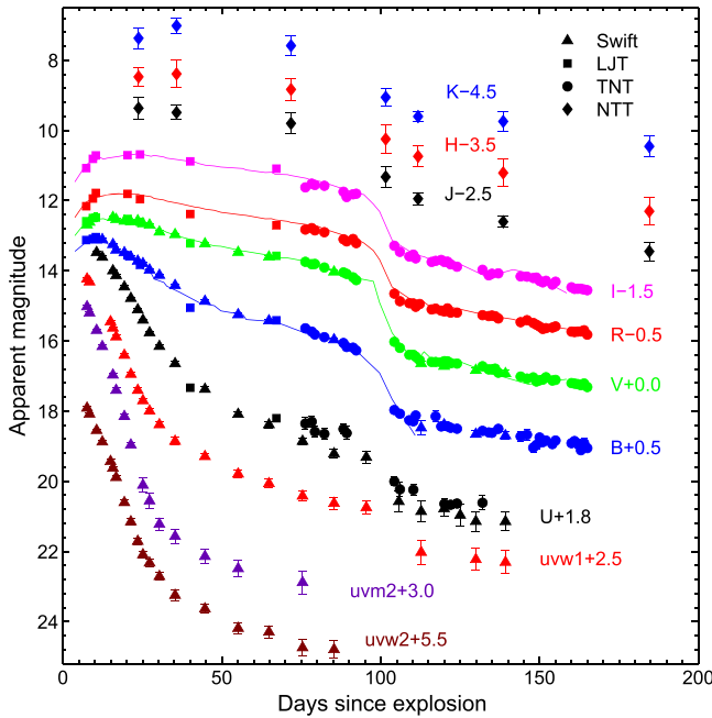
Figure 2. Optical, ultraviolet, and near-infrared light curves of SN 2013ej. The optical data from Richmond (2014) are overplotted as solid lines for comparison. The light curves are shifted in magnitudes for better display. In BVRI bands, the error bars are smaller than the symbols.
