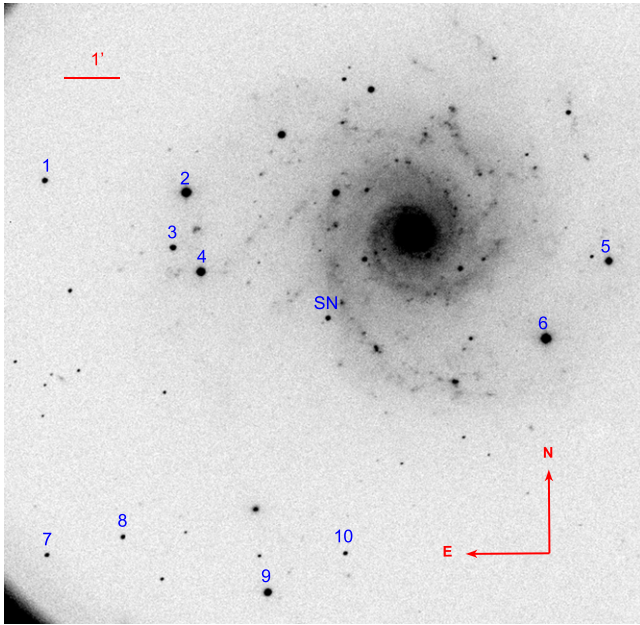
Figure 1. SN 2013ej in M74. The R -band image was taken on 2013 November 7 by the 80 cm Tsinghua-NAOC telescope. The location of the SN and 10 local reference stars are marked. North is up and east is to the left.
