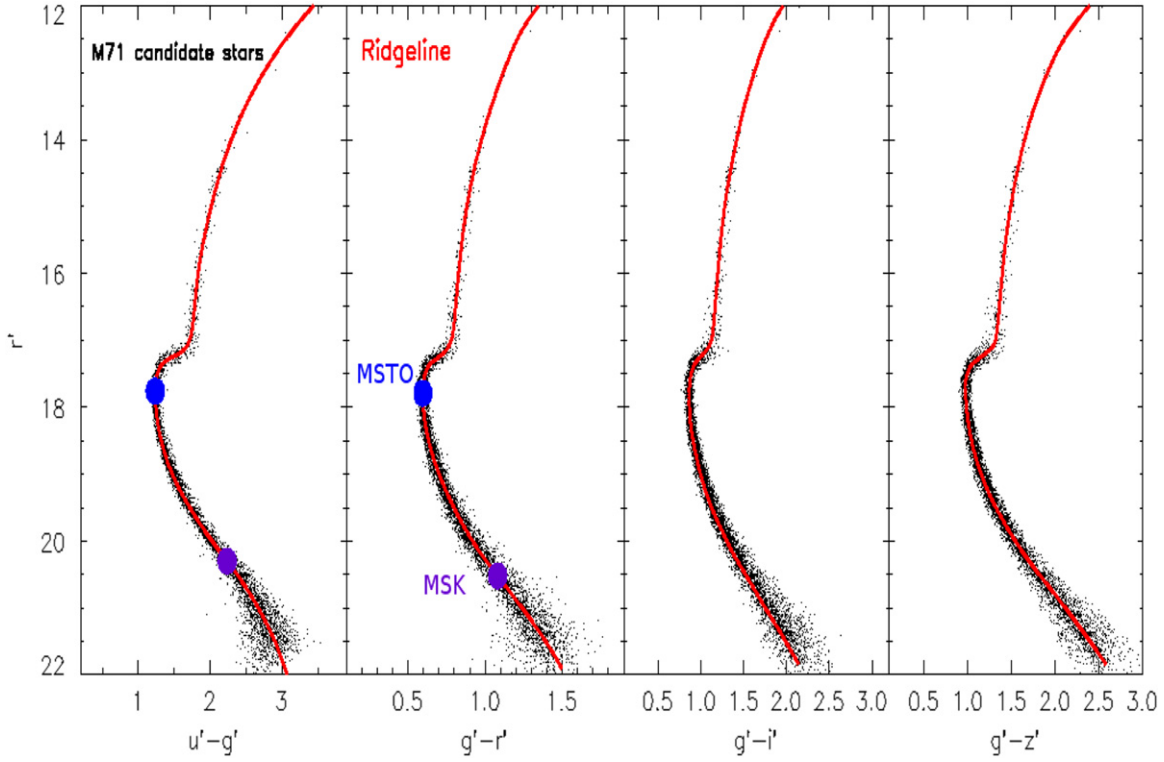
Figure 8. From left to right: optical CMDs of candidate cluster stars. Stars plotted in the different CMDs were selected according to photometric error and cluster radial distance. The red lines display the ridge lines, while the two large blue filled circles plotted in the r' , g' - r' CMD mark the position of both the MSTO and the MSK.
