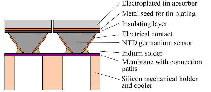
Fig. 1. Schematic structure of the microcalorimeter array.
