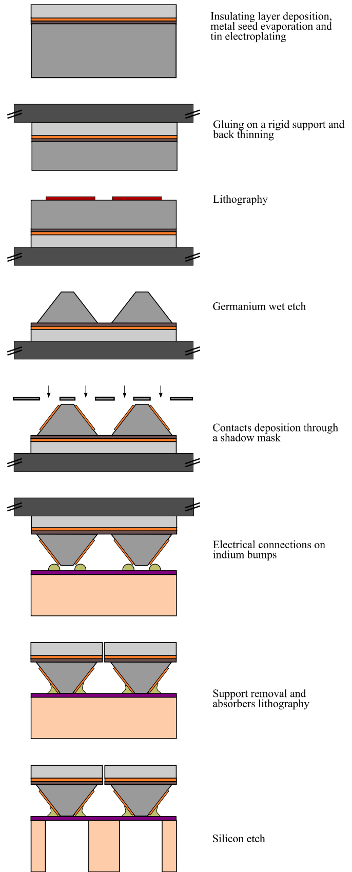
Fig. 2. Schematic view of the main steps of the proposed planar process.
