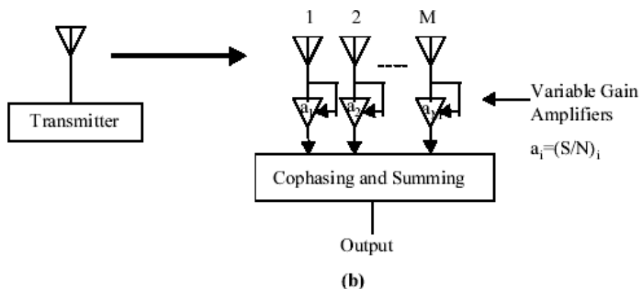
Figure 2.37: Maximal Ratio Combining
