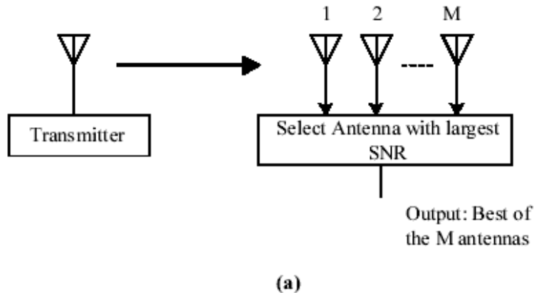
Figure 2.36: Selection diversity
