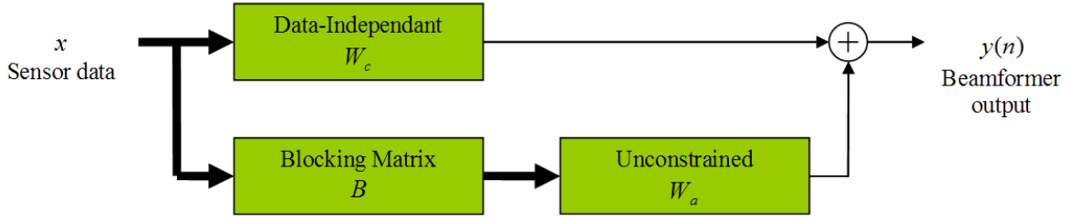
Figure 2.40: Generalized Side lobe Canceller (GSC)
