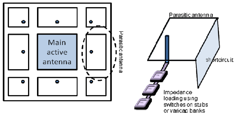
Figure 2.31: SPA MEMtenna concept and detail of the parasitic antenna impedance loading
