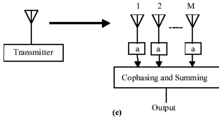
Figure 2.38: Equal Gain Combining
