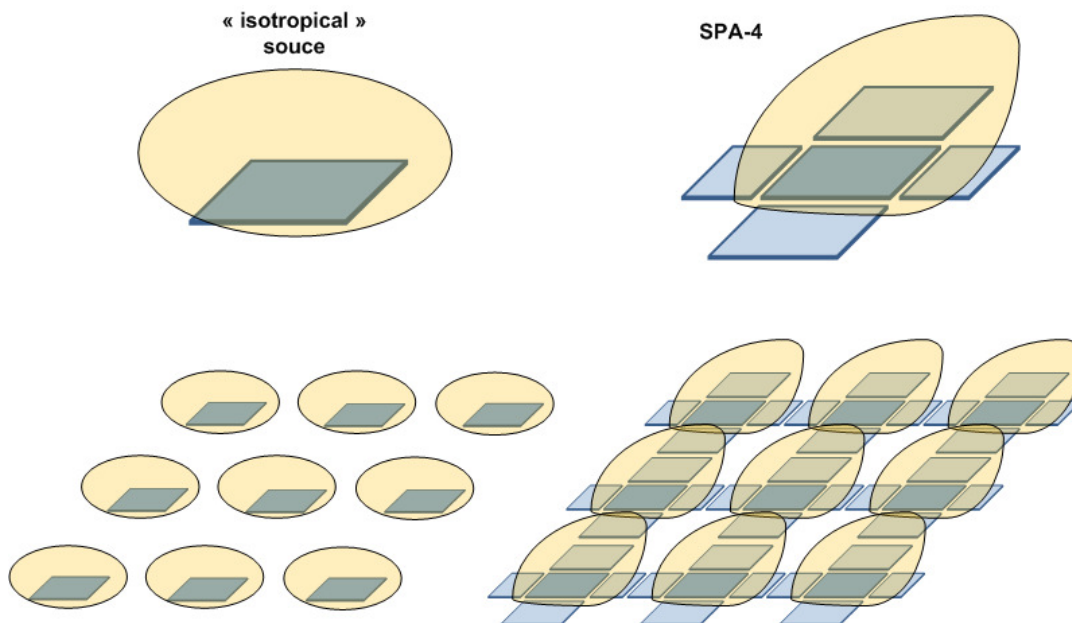
Figure 2.28: 3x3 array using classical “isotropic” sources and SPA-4 array equivalent to parasitic antenna element interleaving
