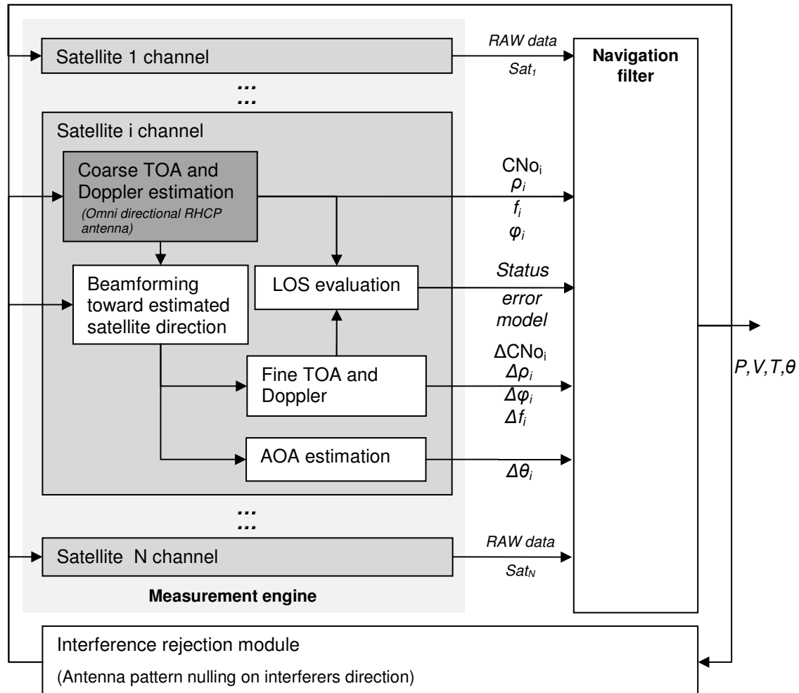
Figure 2.43: Tracking engine and navigation filter processes
