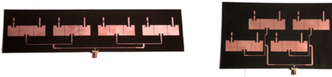
Figure 2.21: Inline and quincunxes WLAN arrays of SPAs
