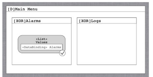
Figure 5: IFML model with one main screen and two internal tabs, to be shown in mutual exclusion.
