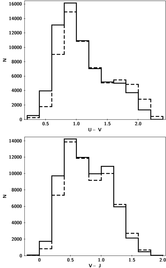
Fig. 2. Distribution of U - V (top panel) and V - J (bottom panel) rest frame colours for the CDFS (solid line) and the COSMOS (dashed line) galaxy samples.
