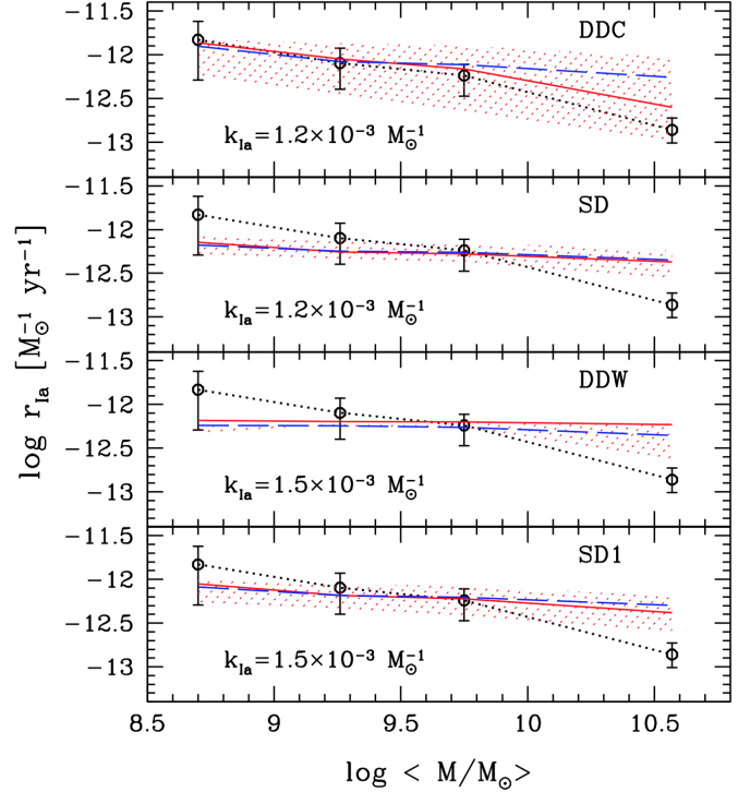
Fig. 16. SN Ia rate as a function of galaxy mass. Black circles are the observed rates in the four mass bins, reported in Table 2, while lines connect the theoretical rates at the median ( \langle \text{Age} \rangle ) of the distributions in the four mass bins. Solid (red) and dashed (blue) lines refer to exponentially declining SFH models with \tau = 0.1 and 8 Gyr, respectively. The shaded areas show the range covered when using the 30th or 70th percentiles of the \langle \text{Age} \rangle distribution instead of the median \langle \text{Age} \rangle , for the exponentially declining SFH models with \tau = 0.1 Gyr.
