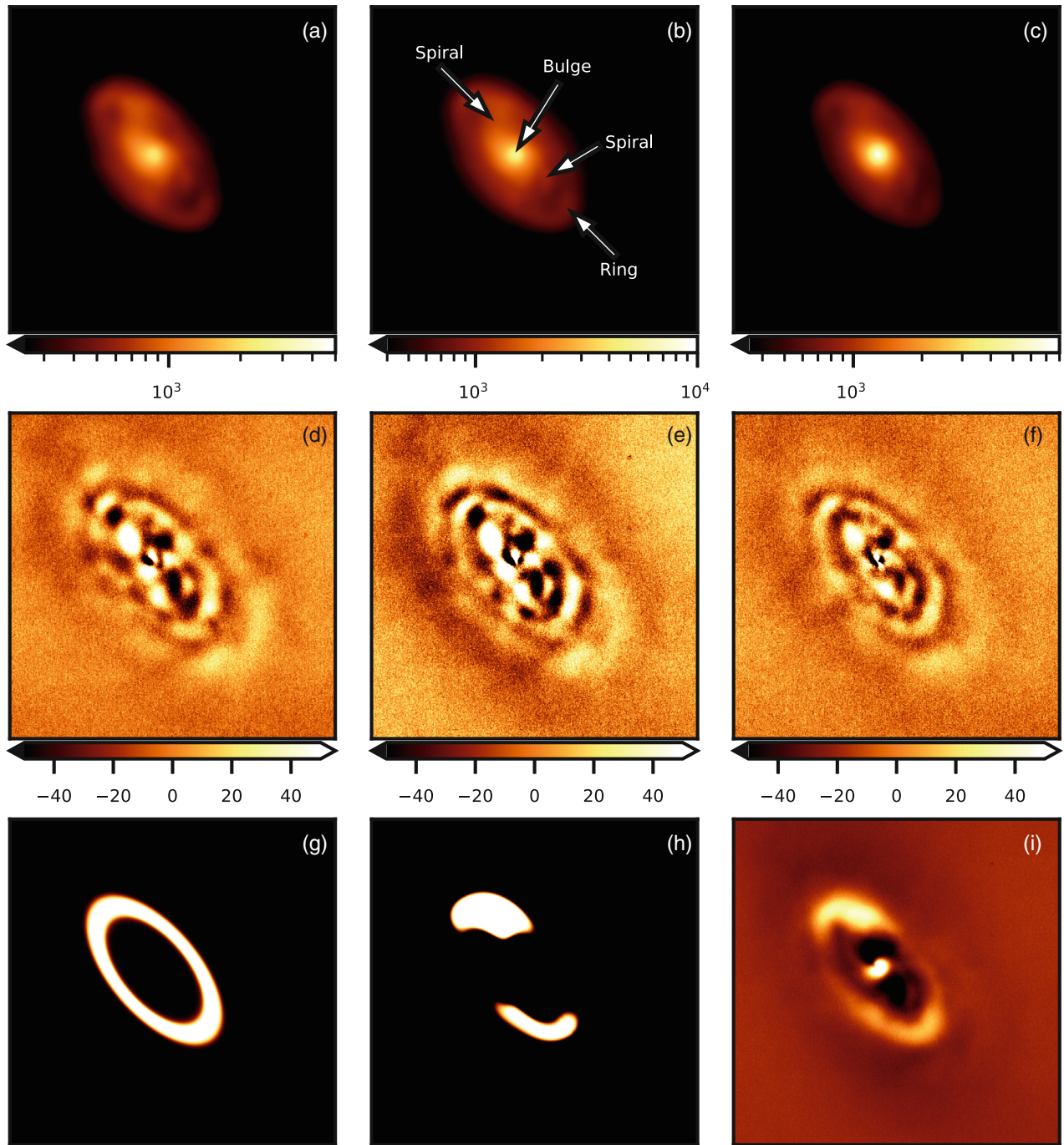
FIGURE 3 (a–c) Cutouts of the central region of NGC 2273 in the J-band (left panel), H-band (middle panel), and Ks-band (right panel). The components that we fitted (or tried to fit) and which we discuss in the text are labeled in the H-band image. (d–f) The residuals after subtraction of the 3-component fit consisting of a bulge, disk, and ring in JHKs ordered like (a–c). (g,h) The simple-ring model and the complex-ring model in the H band. (i) The residual image after subtraction of a one-component disk-fit in the H-band. In each image, the FoV is 9'' \times 9'' . North is up, east is left. Intensities are given in ADU.
