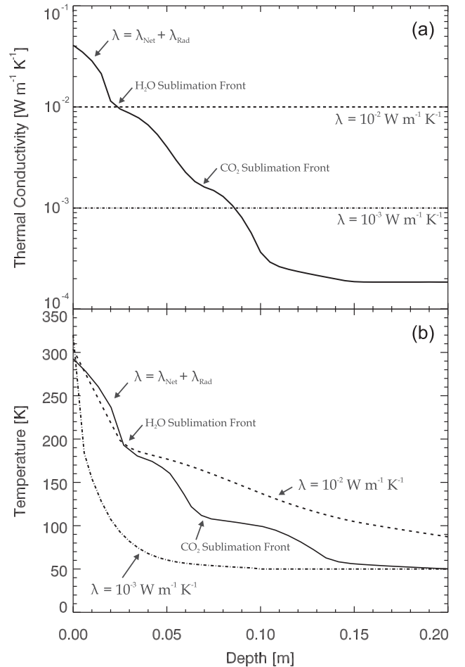
Figure 7. (a) The three heat-conductivity cases used in this study. The dashed and dash-dotted constant heat conductivities represent the homogeneous model, whereas the solid curve characterizes the pebble case in which the radiative heat transfer is important for high temperatures (i.e. for shallow depths) (b) The resulting temperature-depth curves. It should be noted that the dips in the temperature profile are caused by latent cooling due to sublimation. The profiles are extracted 26000 s after the start of the simulation. In the cases of \lambda = \lambda_{\text{Net}} + \lambda_{\text{Rad}} and \lambda = 10^{-2} \text{ W m}^{-1} \text{ K}^{-1} , the \text{H}_2\text{O} sublimation front is located at 0.025 m depth, whereas the \text{CO}_2 sublimation front can be found in deeper layers (at 0.07 m). For comparison, in the low thermal conductivity case ( \lambda = 10^{-3} \text{ W m}^{-1} \text{ K}^{-1} ) less energy is transported into the interior so that the sublimation fronts are still located very close to the surface. It can also be seen that the lower thermal conductivity causes a higher surface temperature.
