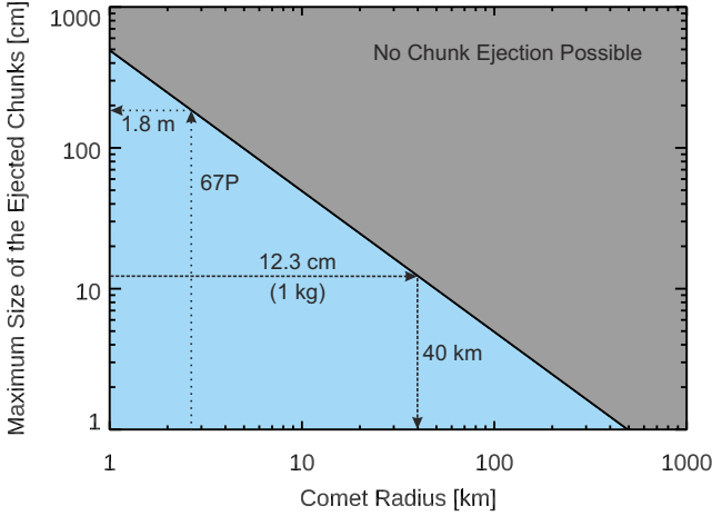
Figure 17. Maximum chunk size that can be detached off a cometary surface as a function of the radius of the nucleus (see equation 6). For these calculations, we assumed \rho_{\text{Comet}} = \rho_{\text{Chunk}} = 532 \text{ kg m}^{-3} and \sigma_T = 0.4 \text{ Pa} . The maximum nucleus radius that is able to eject 1 kg heavy chunks is R_{\text{Comet}} = 40 \text{ km} . Comet 67P is able to eject chunks with sizes up to \sim 2 \text{ m} .
