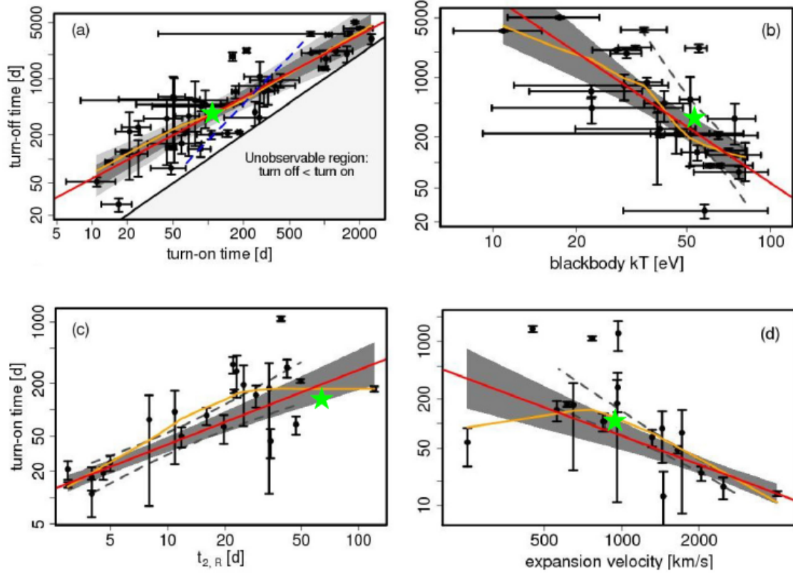
Figure 2: The location of the T Pyx parameters (green stars) with respect to the M31 nova correlations presented in [20]: (1) the t_{on} - t_{off} correlation, for T Pyx measured from the time of maximum brightness; (2) the kT - t_{off} relation, with kT given by the average value kT=55.7 eV; (3) the relation between t_{on} and t_2 and (4) the correlation between t_{on} and the expansion velocity as measured from the H\alpha emission line.
