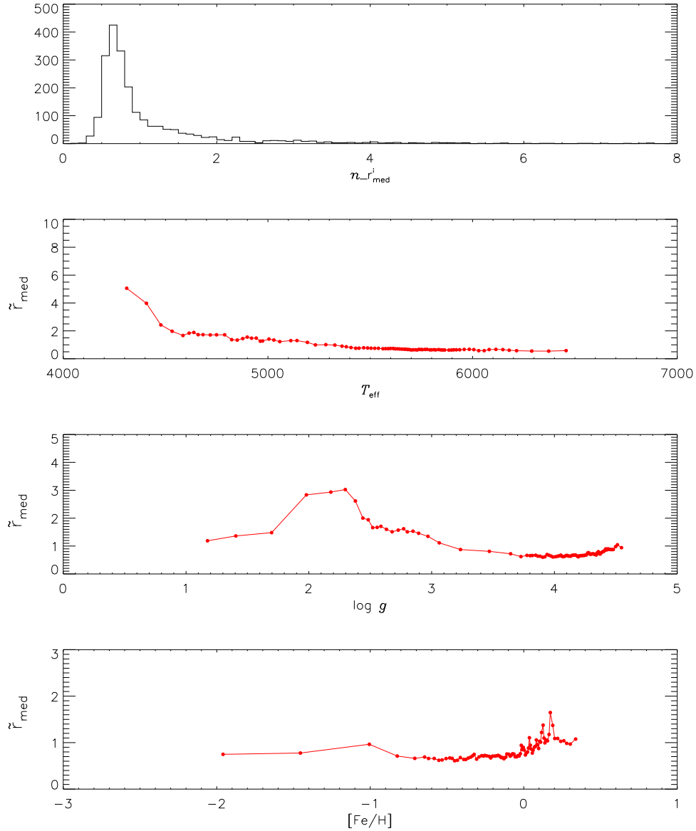
Figure 6. Distribution of n_{r\_med} obtained by using the nominal atmospheric parameter values in computing the synthetic spectra (top panel); the trend of the median values of n_{r\_med} computed in overlapped bins containing 51 stars each vs. T_{eff} , \log g , and [Fe/H] (second, third, and fourth panels respectively).
