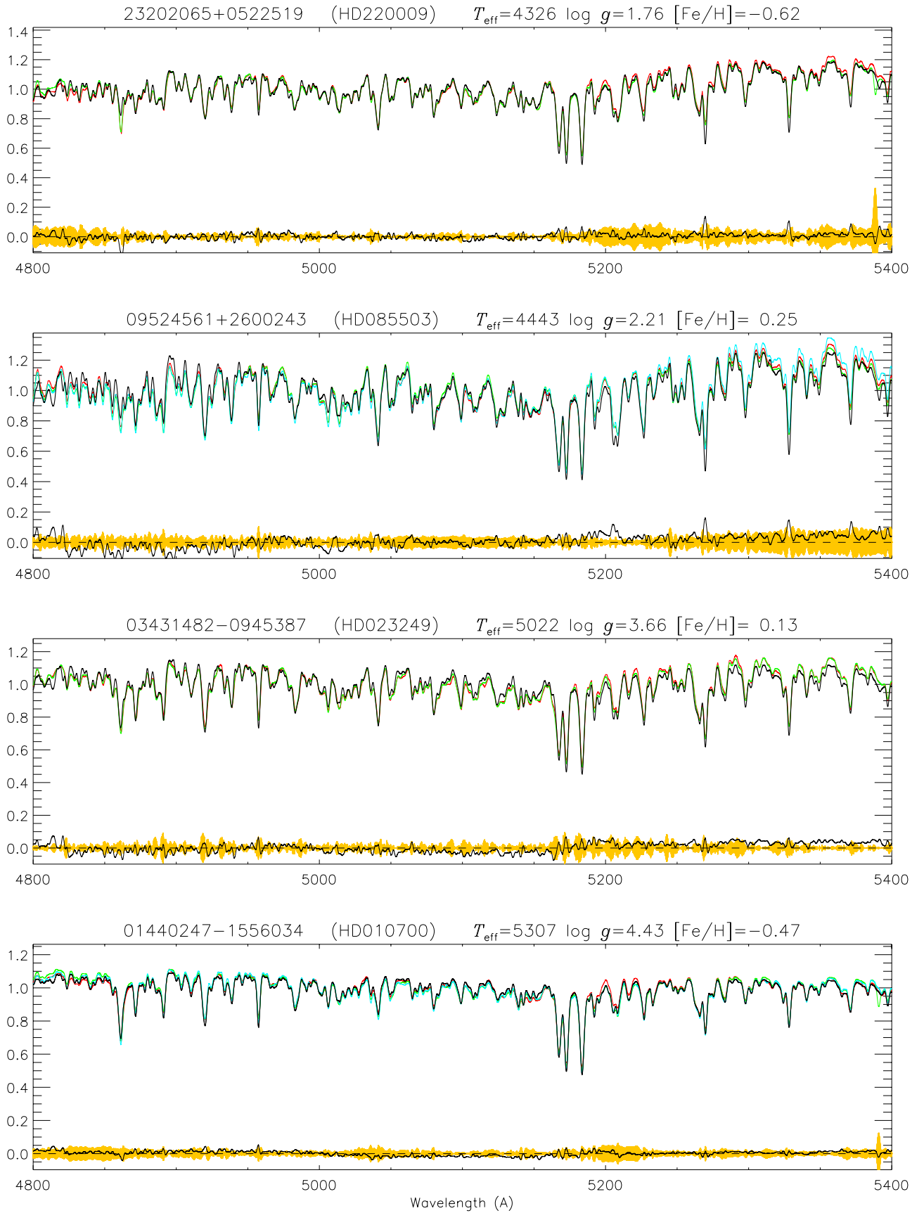
Figure 9. Comparison of flux-calibrated spectra (MILES in red, Indo-US in green, and ELODIE in light blue) scaled according to their median values and the corresponding n_{\text{FSPs}} (black). The black curve at the bottom of each panel shows the flux difference, i.e., the average of the observations minus the corresponding n_{\text{FSP}} , superimposed on the 3\sigma of the observed spectra (yellow area).
