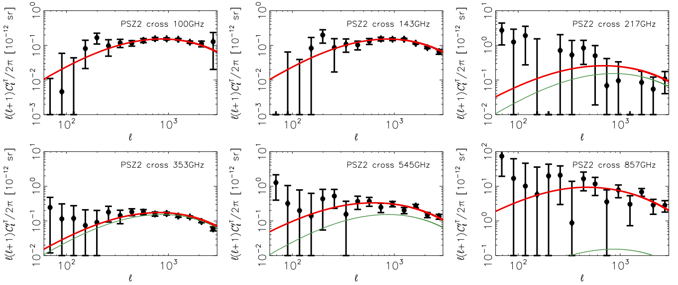
Fig. 12. Observed cross-correlation between the tSZ map ( y_c ) of known clusters and the Planck frequency maps ( T_v ), from 100 to 857 GHz. The data are presented as black circles, the tSZ auto-correlation is in green and the total model y_c - T_v accounting for tSZ-CIB correlation is in red for the best-fit of the CIB and tSZ spectra. All power spectra are presented in Compton-parameter units. Uncertainties are dominated by foreground residuals; thus they are highly correlated from one channel to another.
