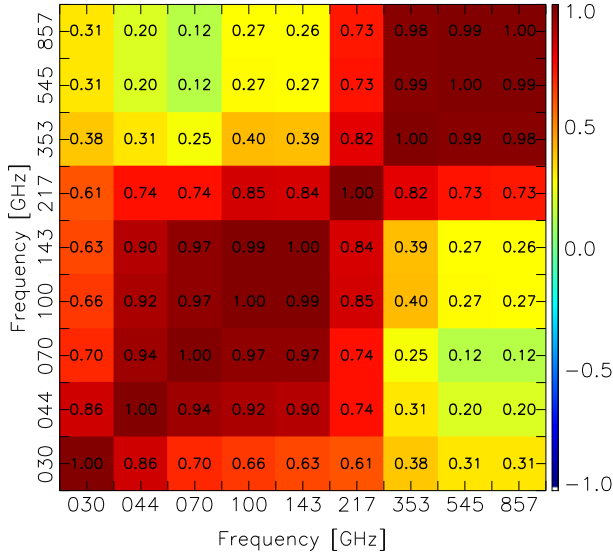
Fig. 9. Correlation matrix of \hat{F}(\nu) estimated from 1000 random positions across the sky.
