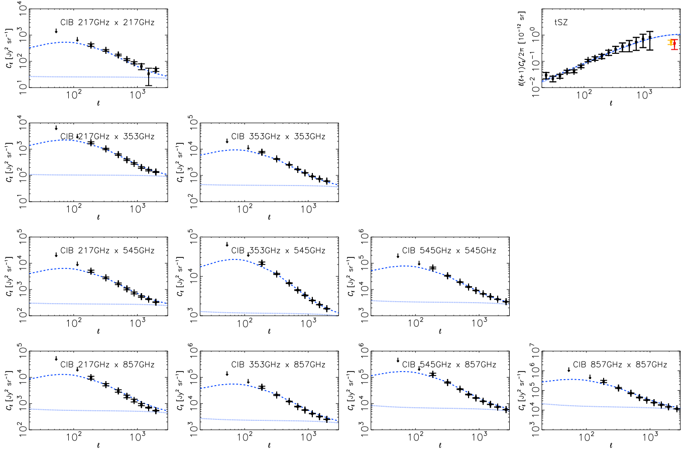
Fig. 5. Upper right panel: observed tSZ power spectrum: Planck data from Planck Collaboration XXI (2014) (black symbols), ACT data Reichardt et al. (2012) (red symbols), and SPT data Sievers et al. (2013) (orange symbols); with our fiducial model (dashed blue line). Other panels: observed CIB power spectra, with Planck data from Planck Collaboration XXX (2014) (black) and our fiducial model (dashed blue line). These panels show auto- and cross-power spectra at 217, 353, 545, and 857 GHz. The dotted blue lines show the 1-halo plus shot-noise term for our fiducial model.
