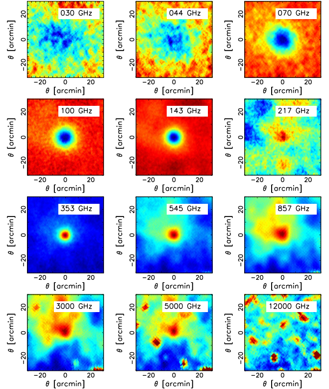
Fig. 6. From left to right and top to bottom: observed stacked intensity maps at 30, 44, 70, 100, 143, 217, 353, 545, 857, 3000, 5000, and 12 000 GHz at the positions of confirmed SZ clusters. All maps are at the native angular resolution of the relevant Planck channel. The measured intensity increases from dark blue to red.
