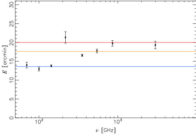
Fig. 11. Variation of the spatial extension, \mathcal{E}(\nu) , of the stacked signal from 70 to 3000 GHz ( 100\ \mu\text{m} ). The blue line shows the expected value for the GNFW profile from Arnaud et al. (2010) and \theta_{500} values from PSZ2, the orange line shows the value we derive with the Xia et al. (2012) profile, and the red line shows the value for an NFW profile with c_{500} = 1.0 .
