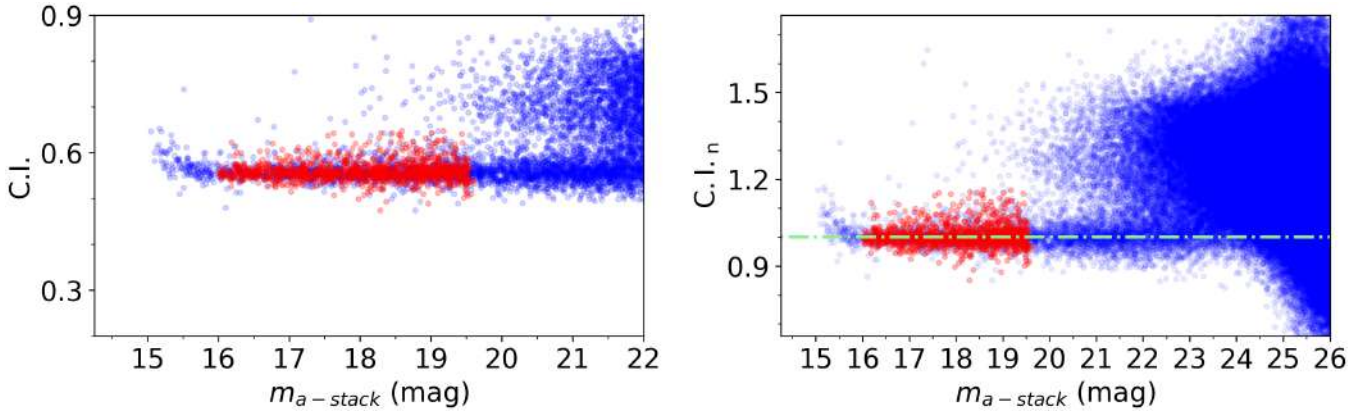
Fig. 6. Normalization procedure for the CI, data for the field FDS#13 are shown. Left panel: concentration index CI = \text{mag}_{4\text{ pix}} - \text{mag}_{6\text{ pix}} versus the uncalibrated a -stack magnitude. For the sake of clarity, only the brightest magnitude range is shown. Blue dots refer to the full sample, red symbols to candidate compact sources used to derive the median CI factor for normalization. Right panel: same as left panel, but over a larger magnitude range and after normalization to the median CI of bright point-like sources (red dots). Point-like sources candidates are aligned along the sequence parallel to the x -axis, around CI_n \sim 1 (green dot-dashed line).
