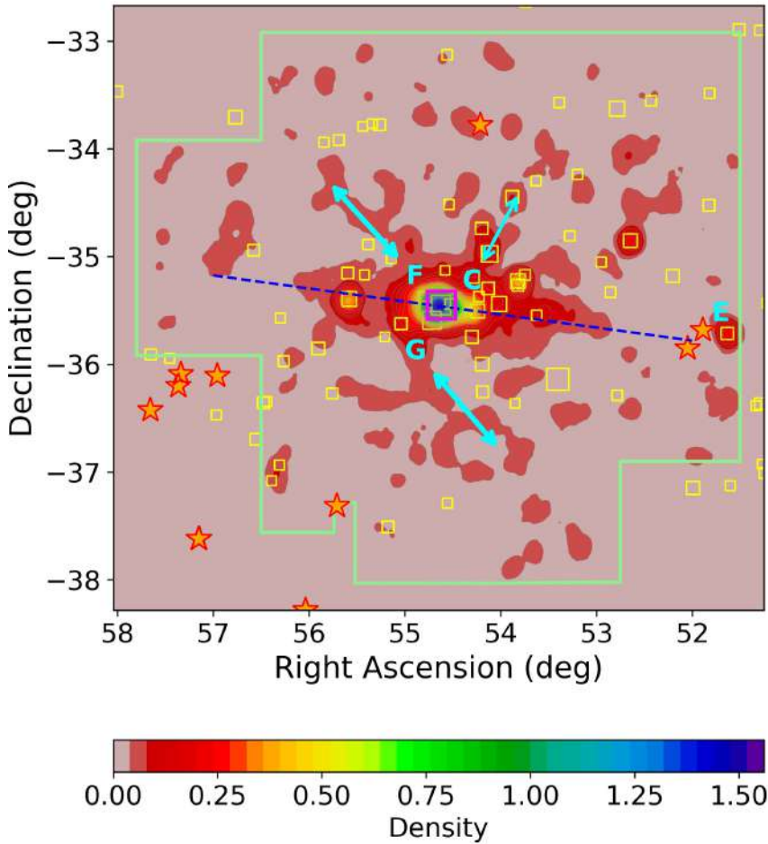
Fig. 11. Single-panel view of the 2-D GC surface density distribution. Iso-density contours and symbols are the same as in Fig. 10 (third contour level plots). Light blue arrows and labels indicate the GC overdensities discussed in the text. The blue dashed line shows the \sim 10^\circ tilt in the direction of NGC 1336 (“E” label in the figure).
