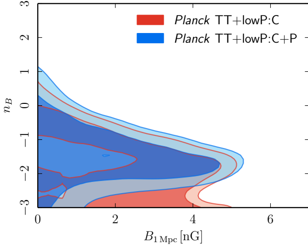
Fig. 8. PMF amplitude versus the spectral index for the baseline Planck 2015 case. C+P denotes the case where both compensated and passive modes are considered, whereas C indicates the case with only compensated modes. The two contours represent the 68 % and 95 % confidence levels.
