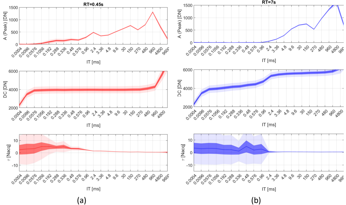
FIG 19 Images show the three parameters A , D , \tau for all the IT commanded for low RT=0.45 in a and for RT=7s in b.. The plots show the trend, the standard deviation associated (dark red) and 3 times the same value (light red). In a er reported the measurement
