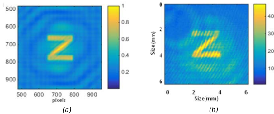
Fig. 14: Reconstruction of a 720x720 pixels stepped CGH, of a 200x200 pixels “Z” of 2x2mm at a focus of 2m (a) Simulation of the reconstruction from theoretical CGH (b) Real reconstruction of the image
