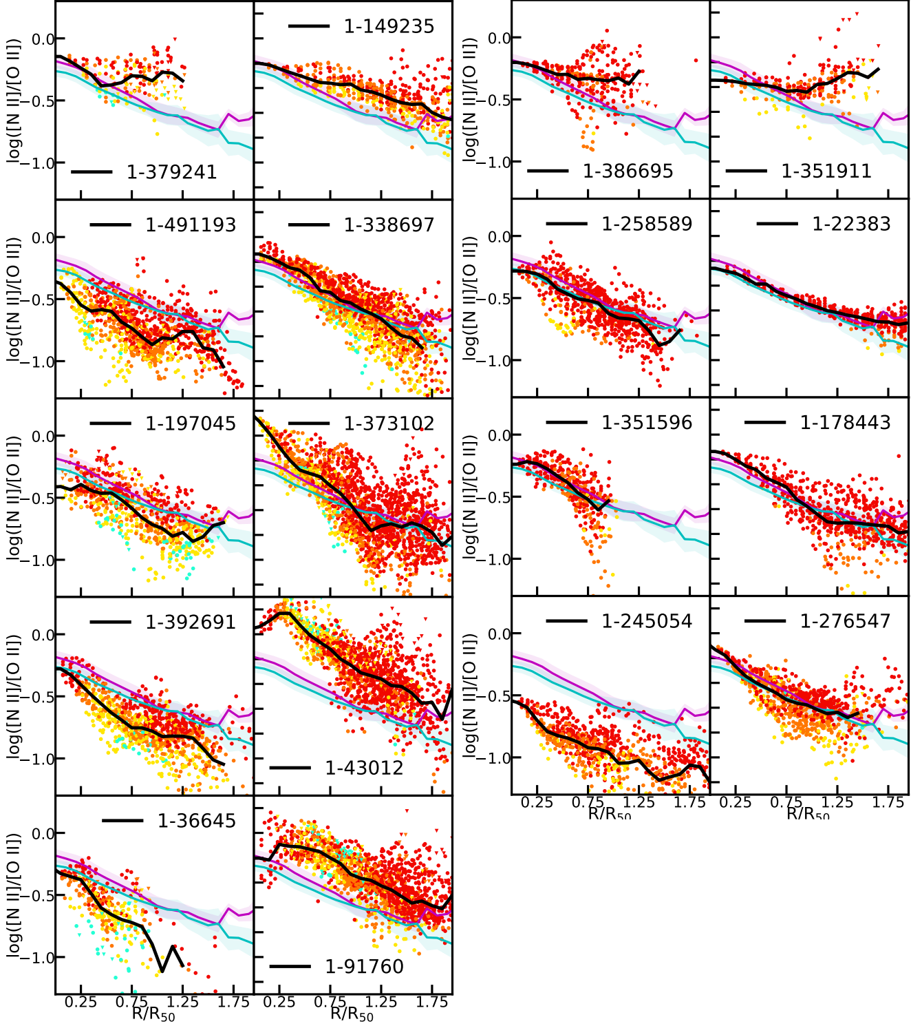
Figure A2. Radial profiles of [N II]/[O II] of each galaxy belonging to QG sample (left) and to SF sample (right). See Figure A1 for panels description.
