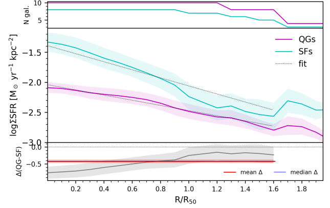
Figure 15. The SFR surface density ( \log \Sigma\text{SFR} ) radial profile for QG and SF samples. The dotted black lines represent the linear fit to the radial profiles. The layout of the figure is the same as in Figure 10.
