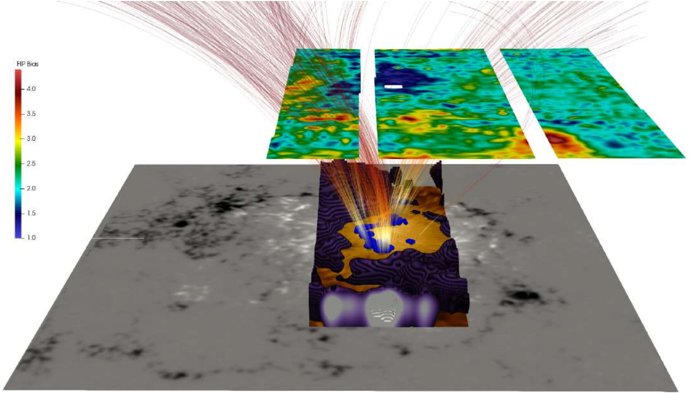
Fig. 2. Three-dimensional view of the AR 12546. From bottom to top: SDO/HMI magnetogram, IBIS Fe I core with blue dots overplotted, and Hinode/EIS FIP bias map. The purple surface represents the equipartition layer ( 0.8 < c_s/v_A < 1.2 ) as inferred from the spectropolarimetric inversions. Selected field lines from a PFSS extrapolation of the coronal field link the blue dots with regions of high-FIP bias on the eastern and southern edges of the sunspot (i.e., in the penumbra; see Baker et al. 2021 for more details).
