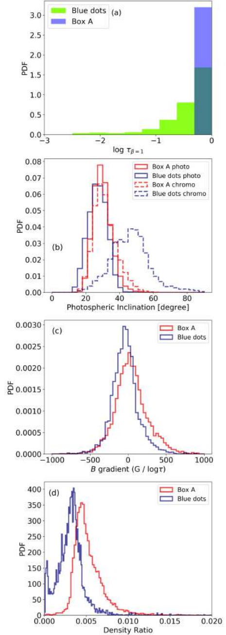
Fig. 4. Panel a: PDF of the optical depths, \log_{10}(\tau) , corresponding to the equipartition layer ( v_A = c_s ) associated with the locations of the blue dots and the area inside box A shown in Fig. 1f. Panel b: PDFs of the magnetic field inclination angles at photospheric ( \log_{10}(\tau) = -1.0 , red and blue histograms) and chromospheric ( \log_{10}(\tau) = -4.6 ; dashed histograms) heights. Panels c and d: PDF distribution of the magnetic field gradient and density ratio for the selected region (i.e., the blue dots and box A).
