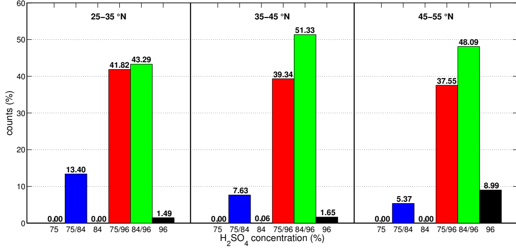
Figure 14: Percentage counts of the distribution of the retrieved sulphuric acid concentrations. Results are plotted for three latitudinal bands. Double values in the abscissa refer to the concentration of the upper and the lower cloud respectively.
